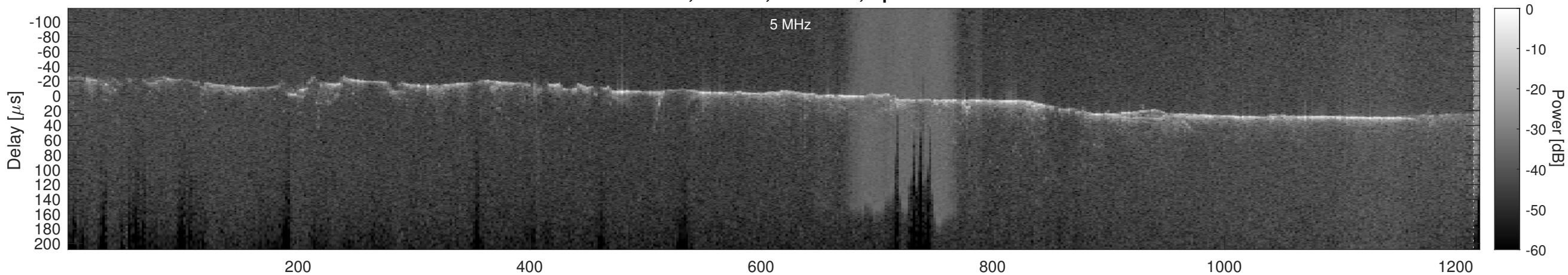
Orbit 23039, Cluttergram
