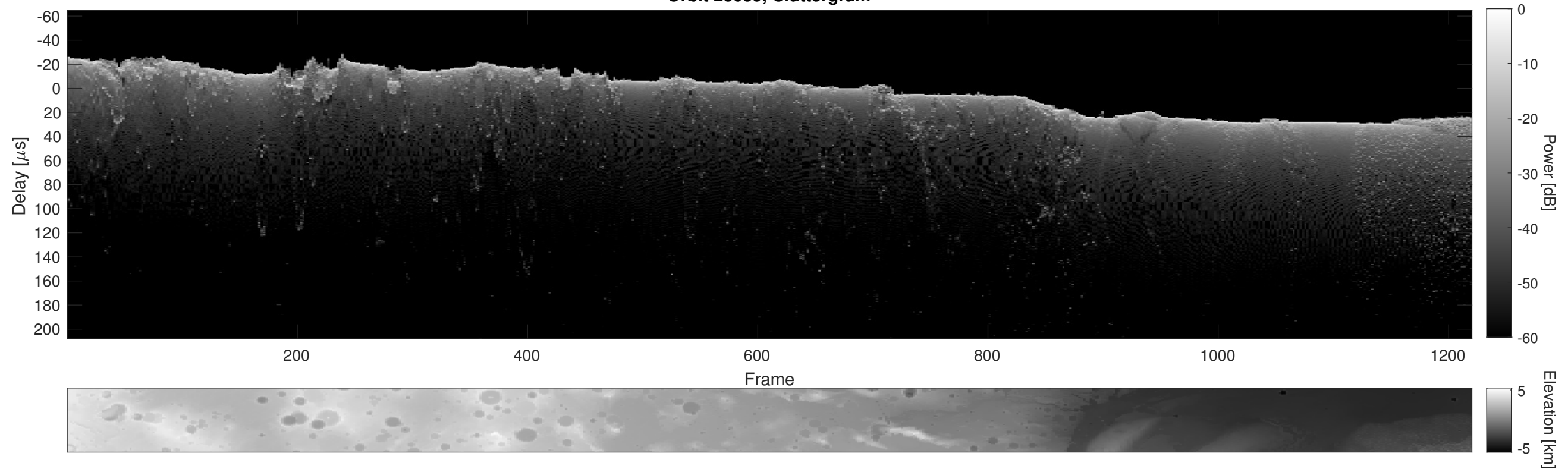
Orbit 23039, Cluttergram
