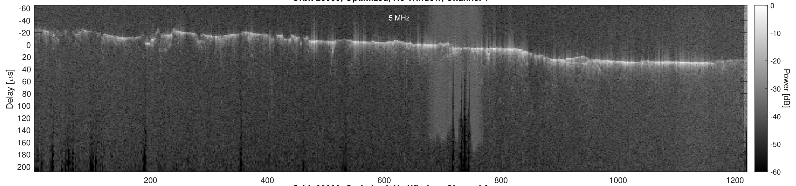
Orbit 23039, Optimized, No Window, Channel 2
