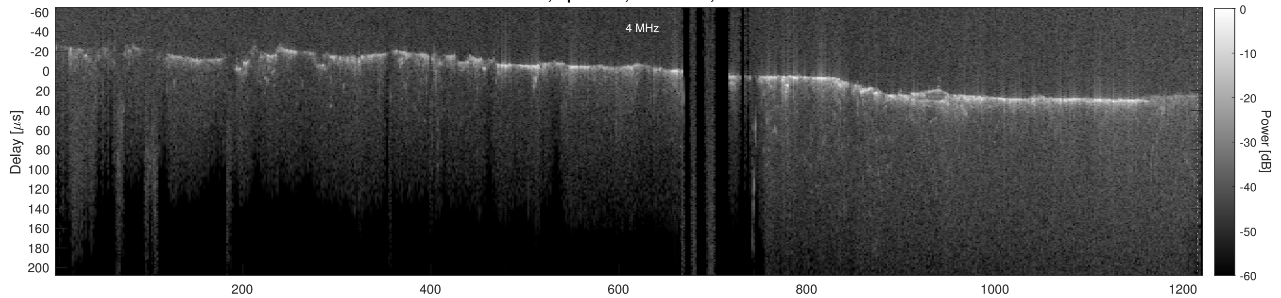
Orbit 23039, Cluttergram
