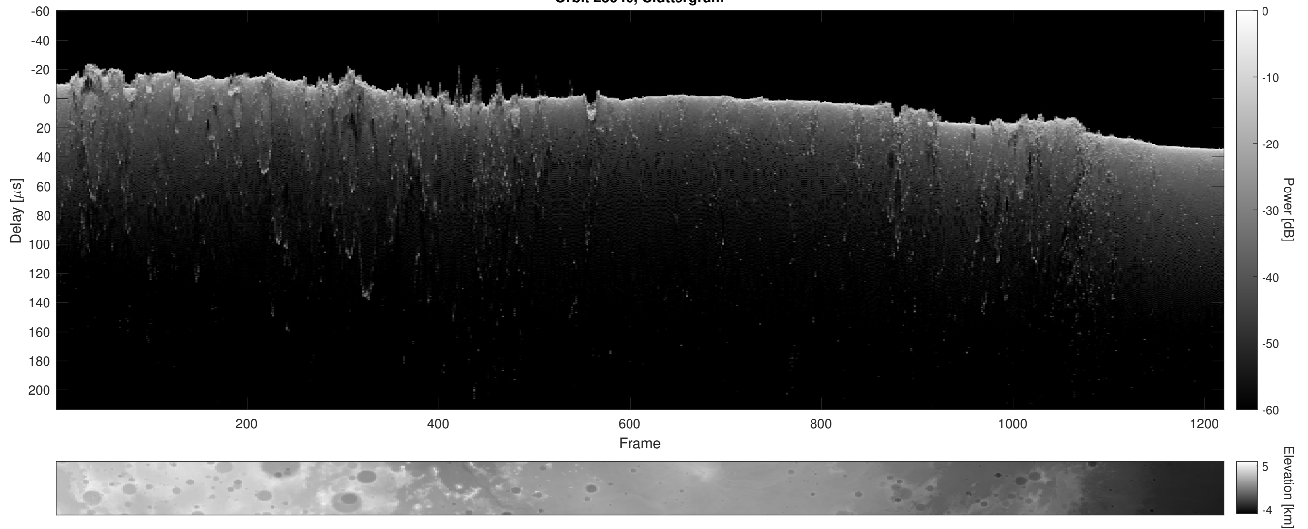
Orbit 23040, Cluttergram
