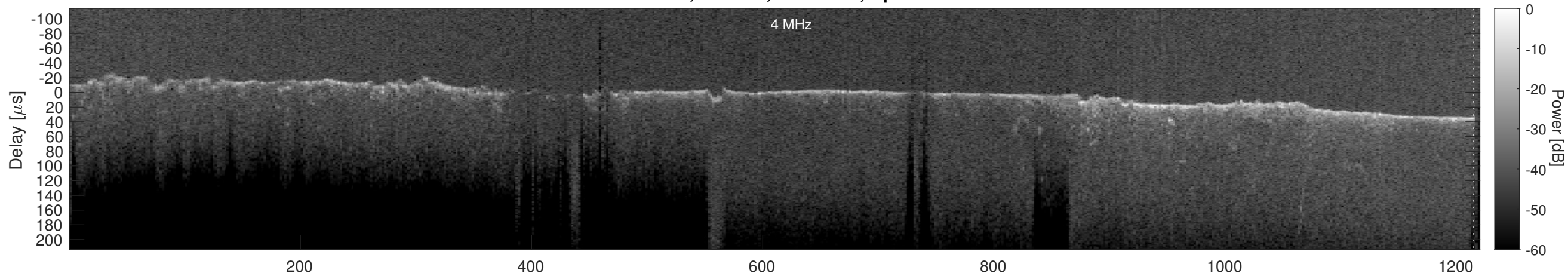
Orbit 23040, Cluttergram
