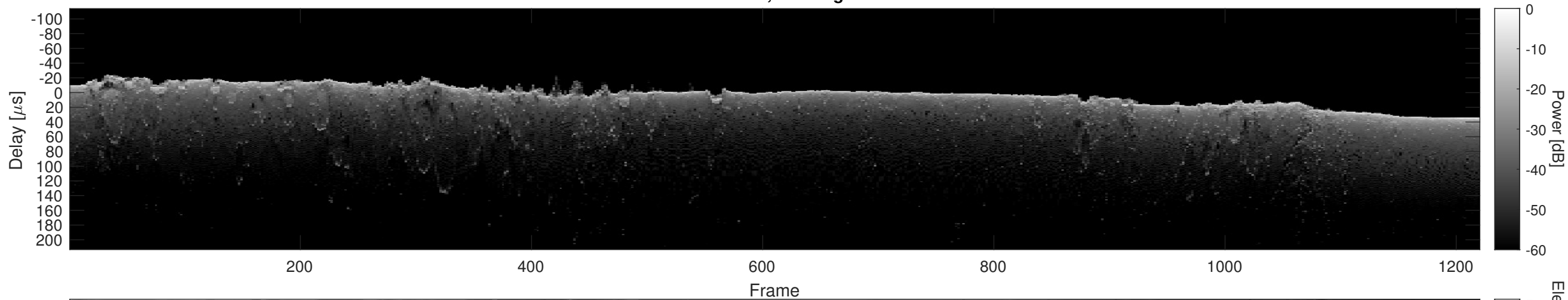
Orbit 23040, Cluttergram
