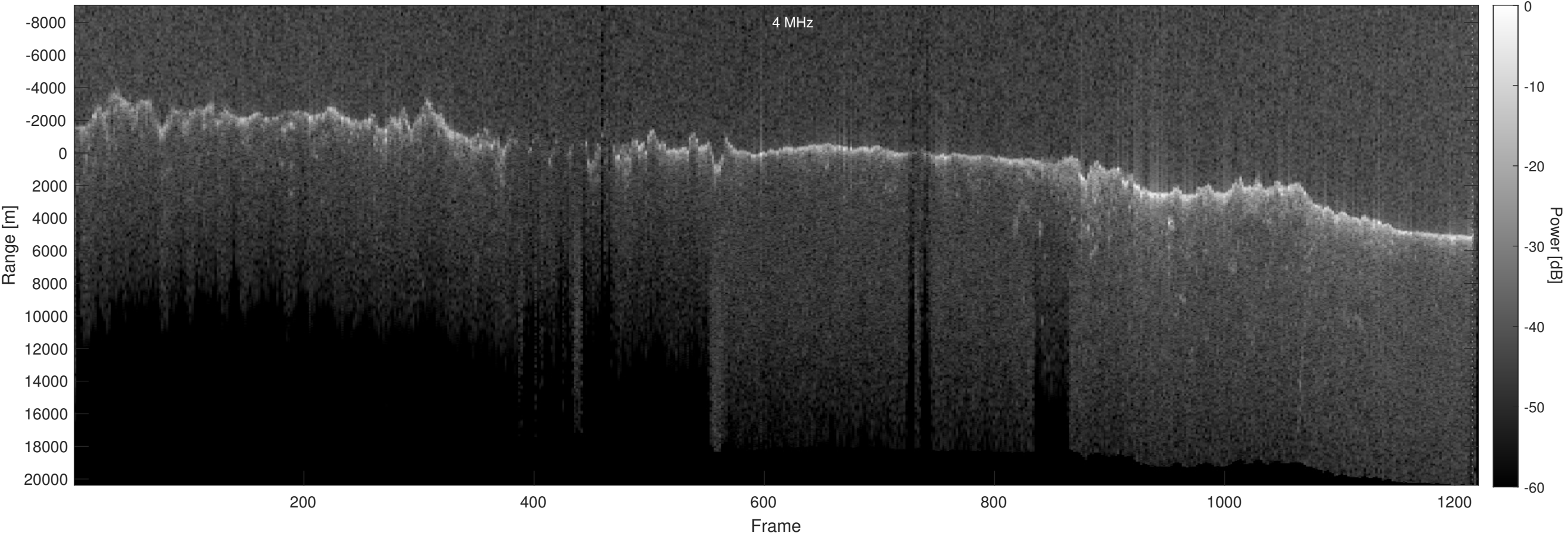
Orbit 23040, Optimized, No Window, Depth-Corrected, Channel 2
