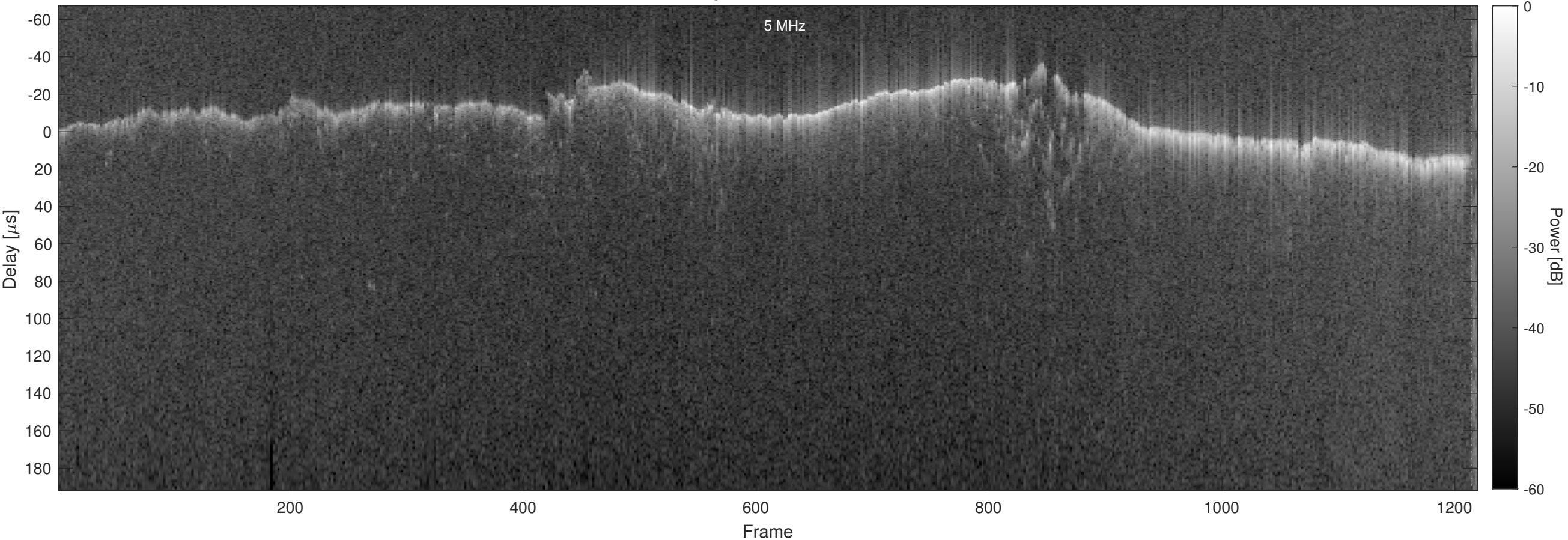
Orbit 23042, Chapman, No Window, Channel 2
