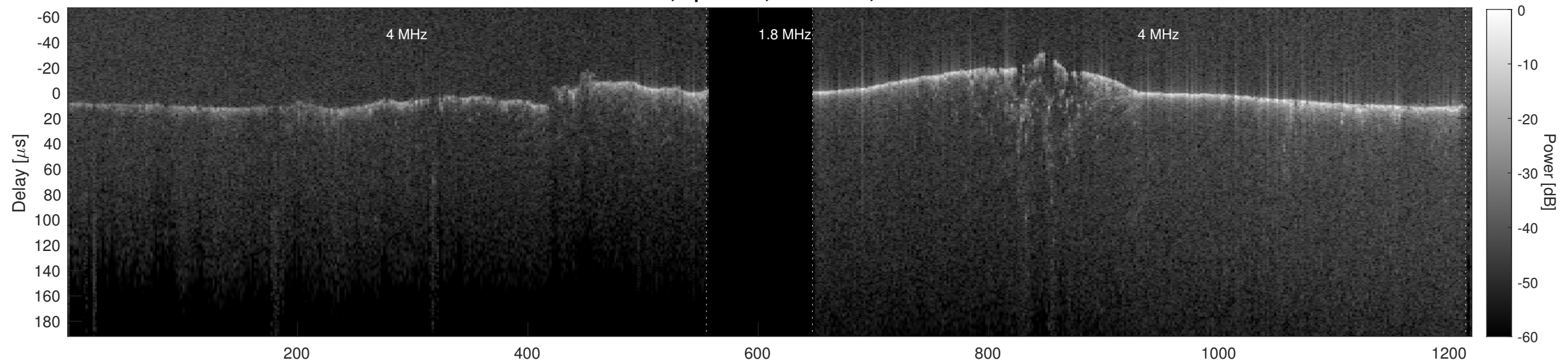
Orbit 23042, Cluttergram
