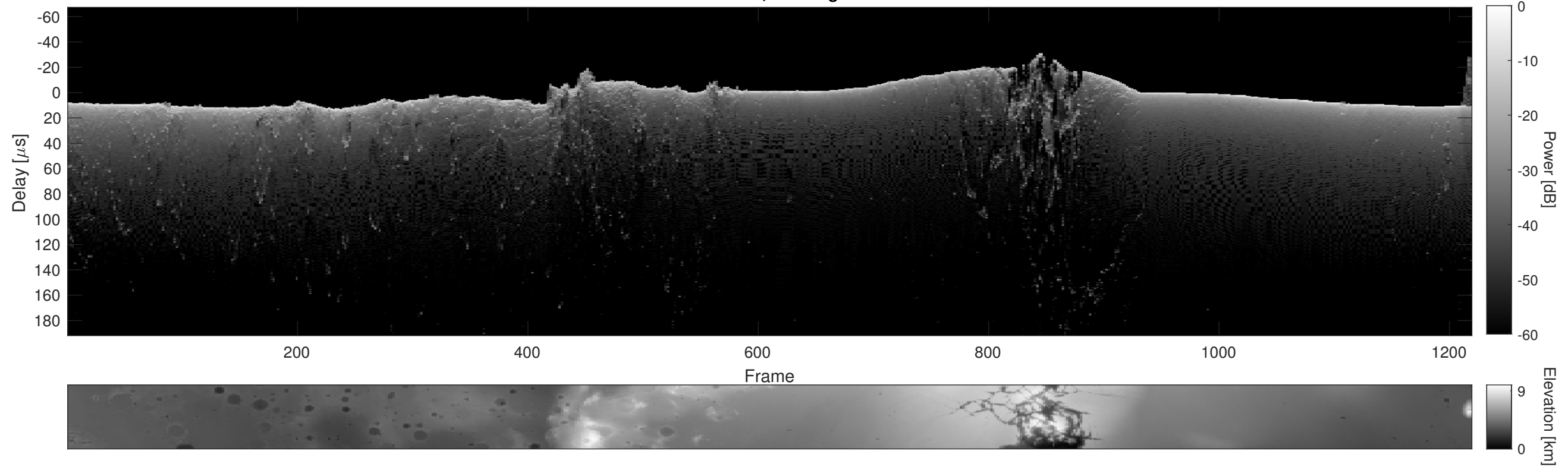
Orbit 23042, Cluttergram
