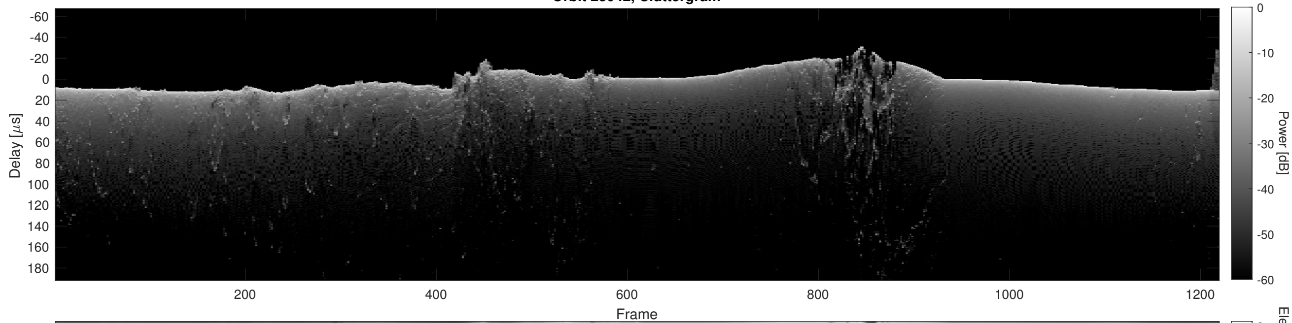
Orbit 23042, Cluttergram
