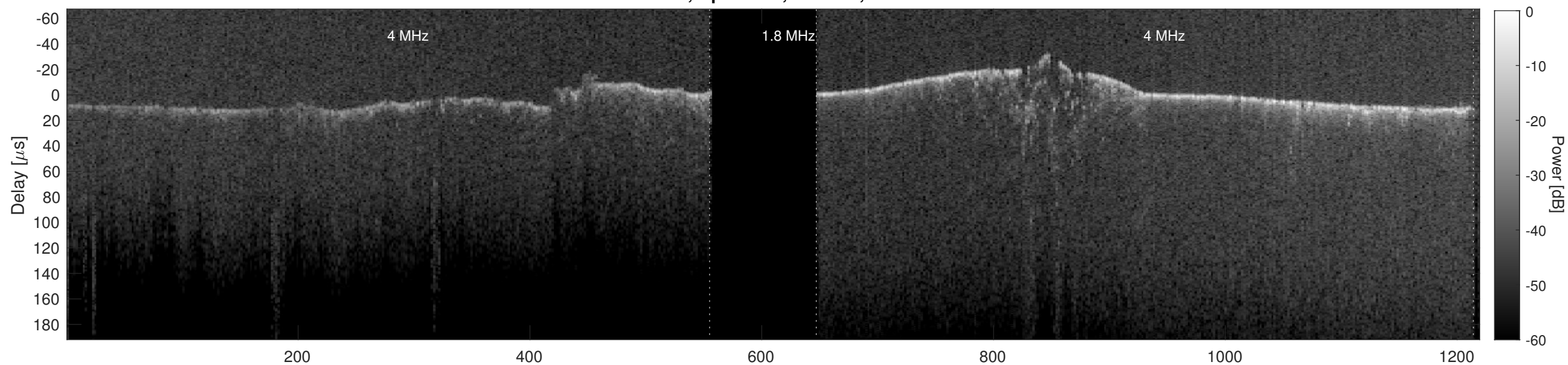
Orbit 23042, Cluttergram
