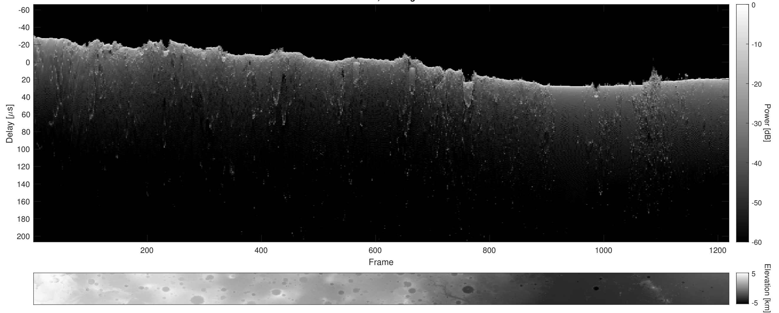
Orbit 23043, Cluttergram
