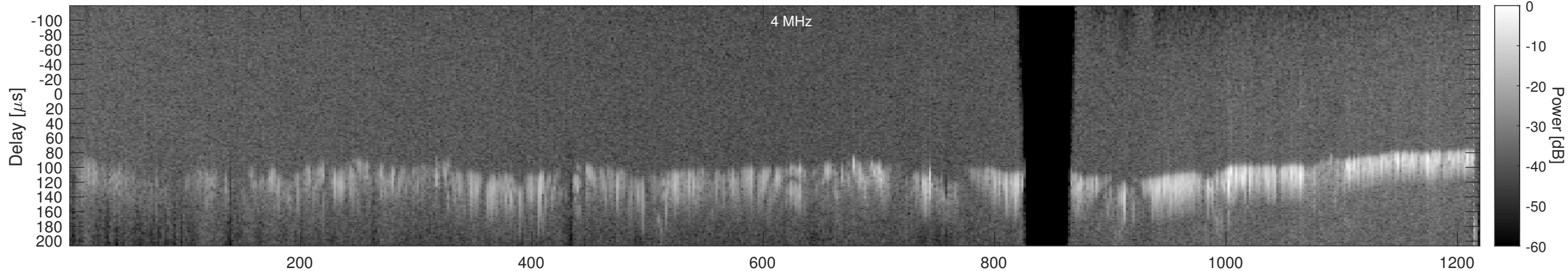
Orbit 23043, Window, Channel 2, Chapman
