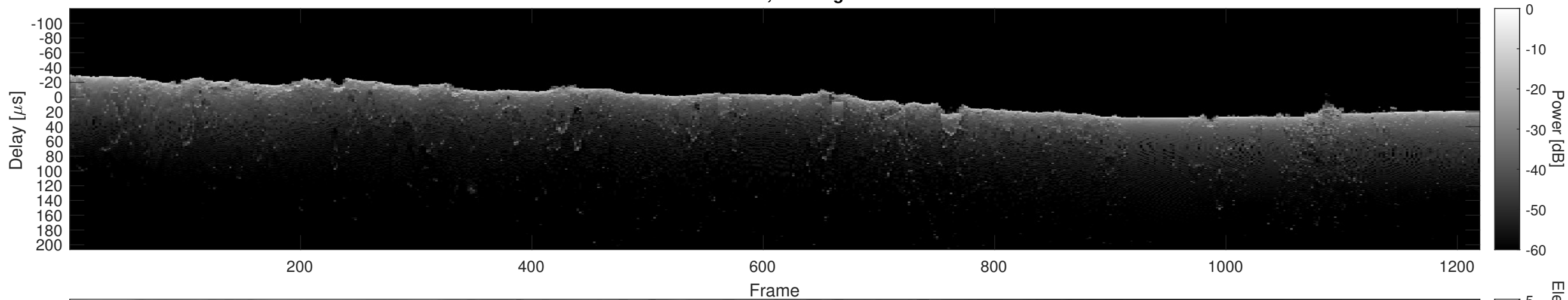
Orbit 23043, Cluttergram
