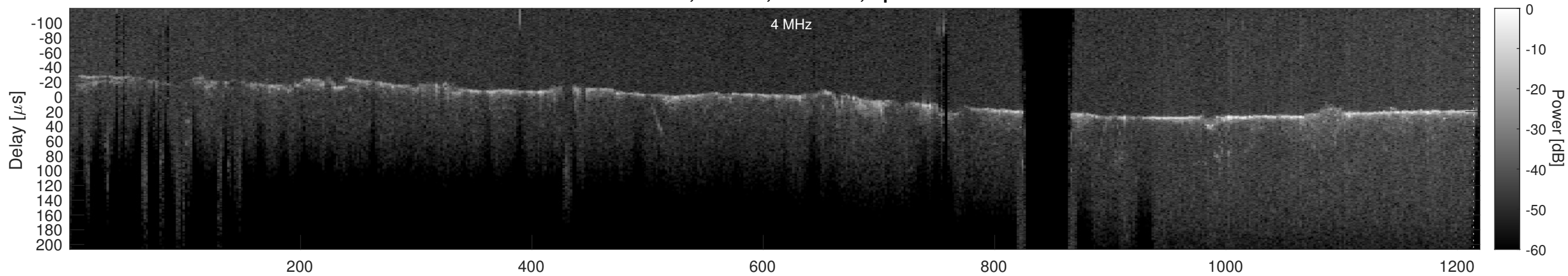
Orbit 23043, Cluttergram
