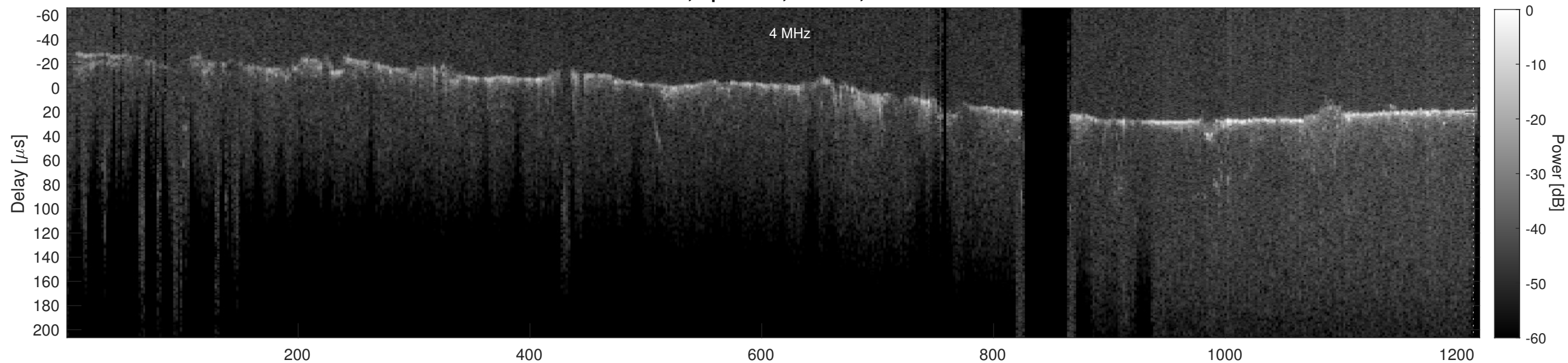
Orbit 23043, Cluttergram
