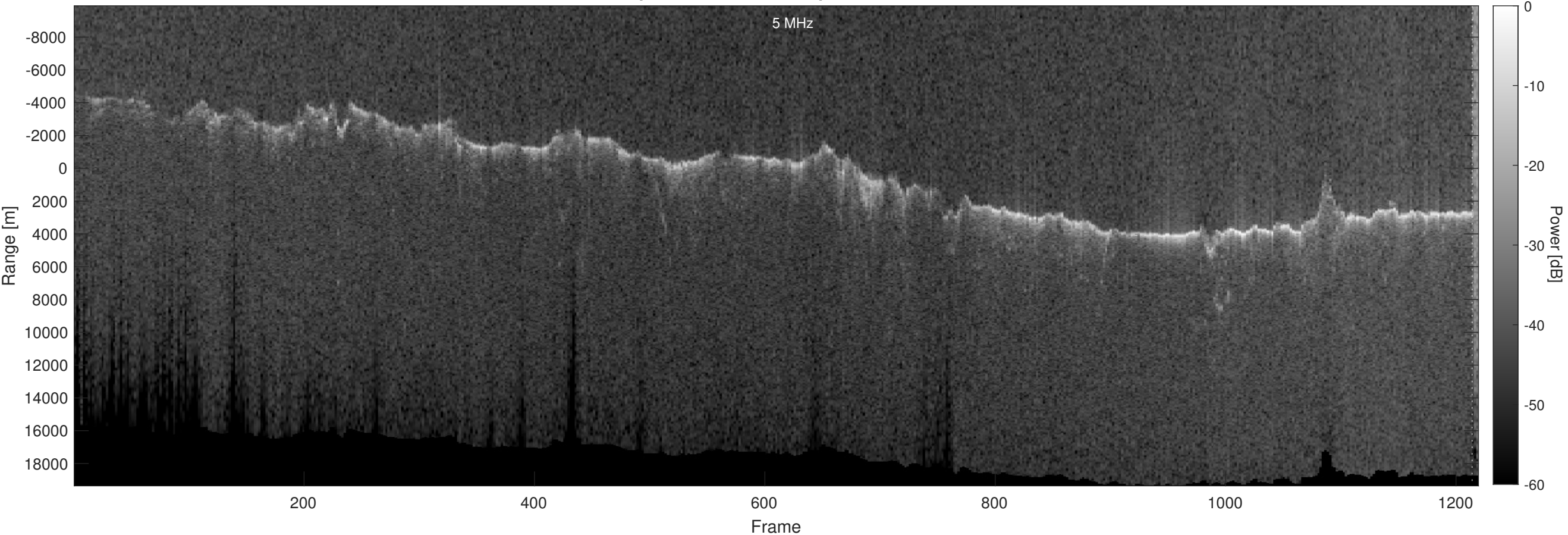
Orbit 23043, Optimized, Window, Depth-Corrected, Channel 2
