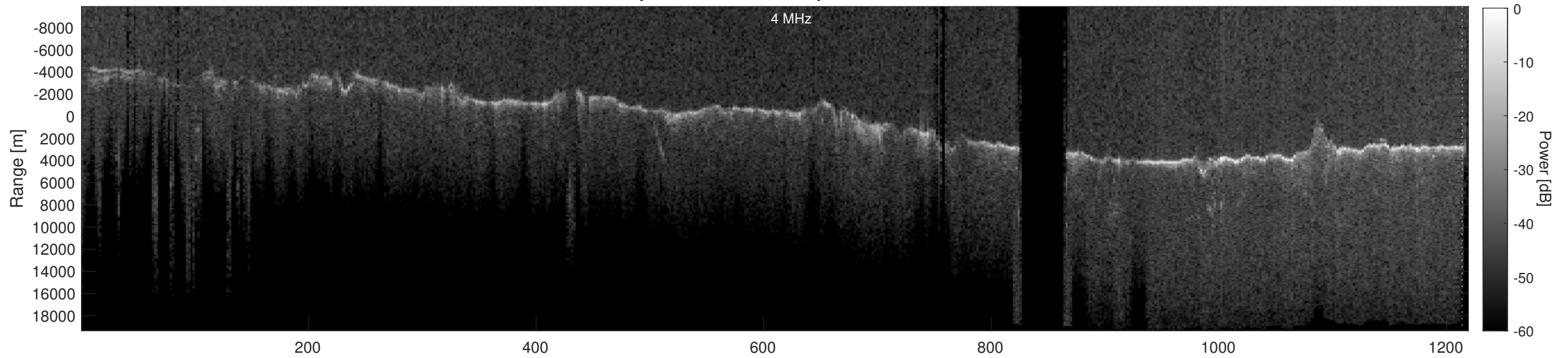
Orbit 23043, Depth-Corrected Cluttergram
