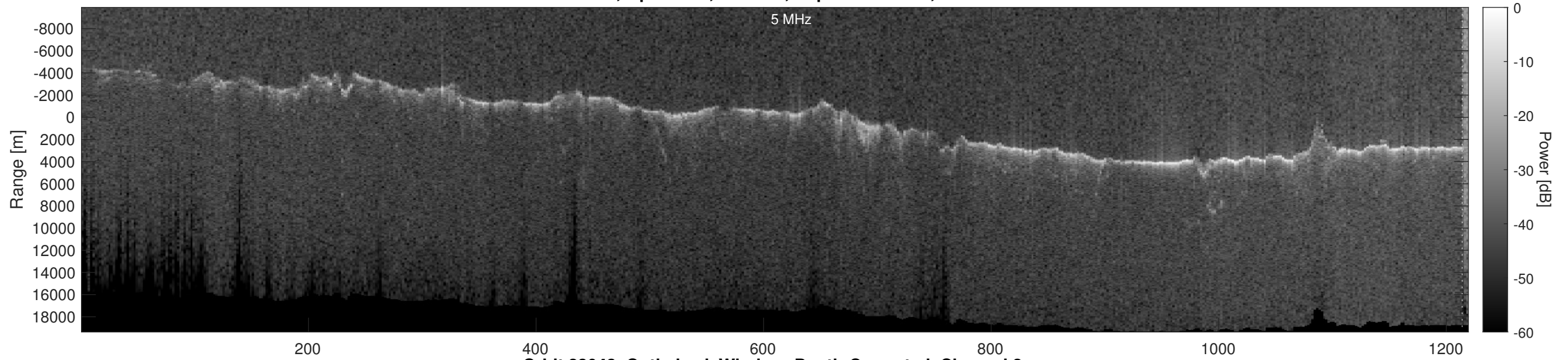
Orbit 23043, Optimized, Window, Depth-Corrected, Channel 2
