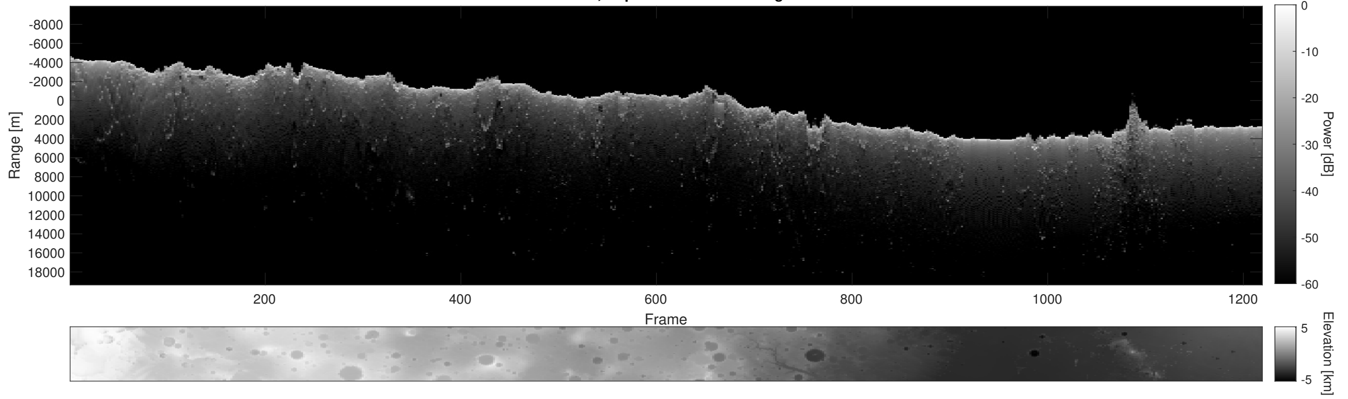
Orbit 23043, Depth-Corrected Cluttergram
