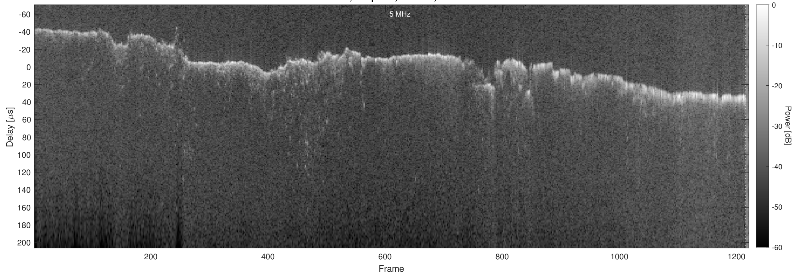
Orbit 23045, Chapman, Window, Channel 2
