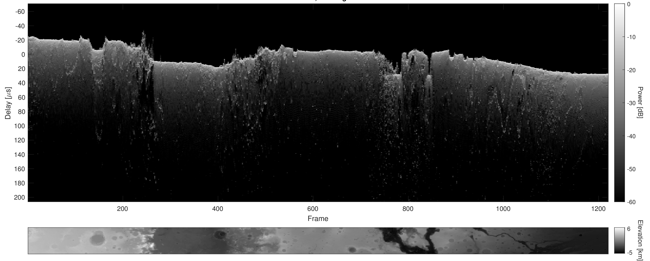
Orbit 23045, Cluttergram
