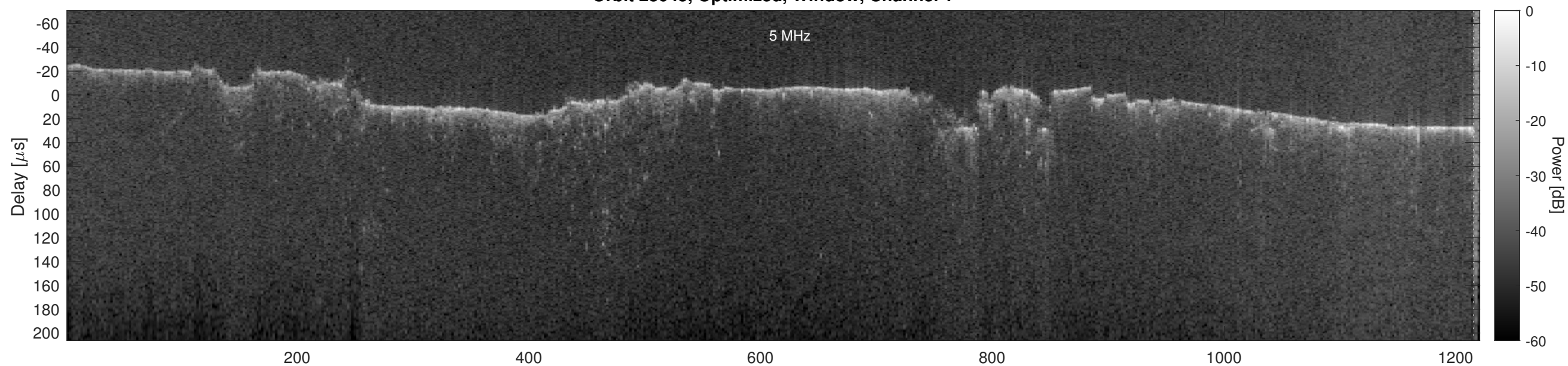
Orbit 23045, Optimized, Window, Channel 2
