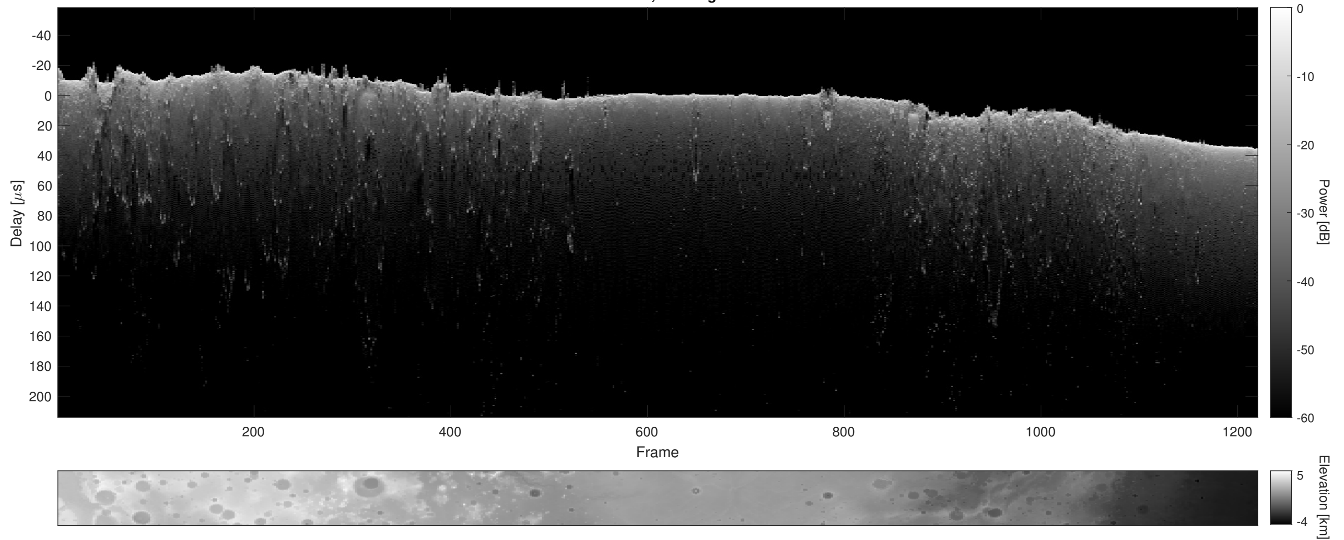
Orbit 23047, Cluttergram
