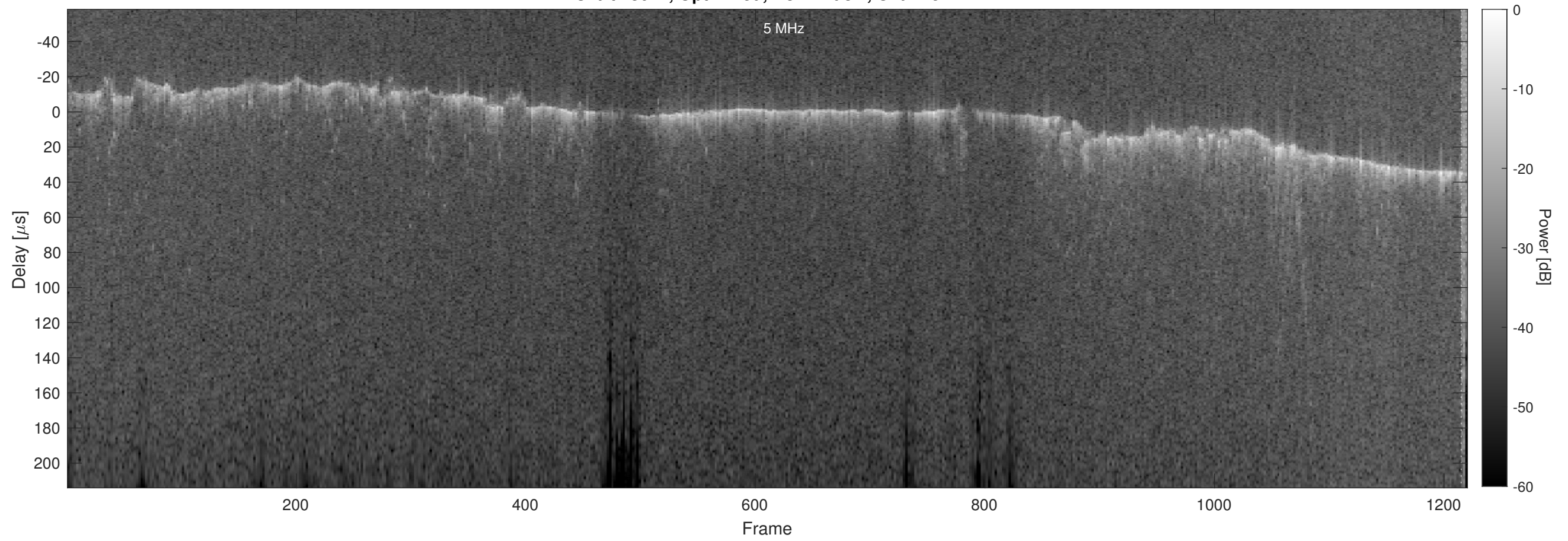
Orbit 23047, Optimized, No Window, Channel 2
