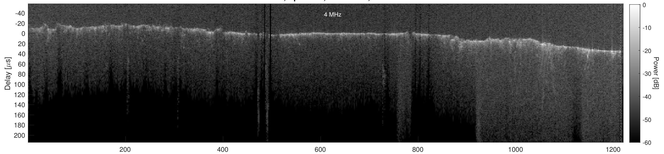
Orbit 23047, Cluttergram
