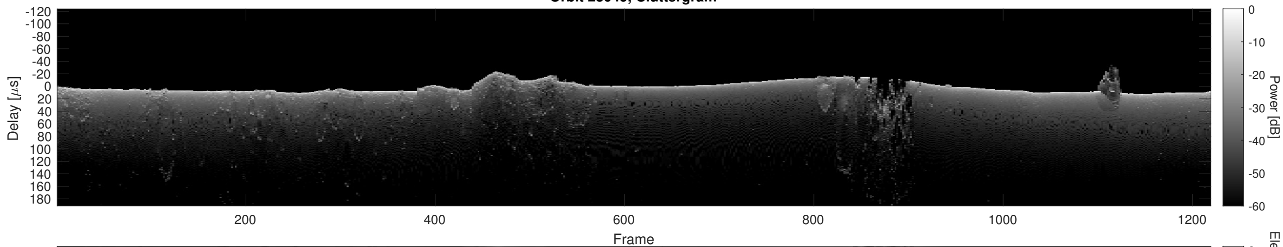
Orbit 23049, Cluttergram
