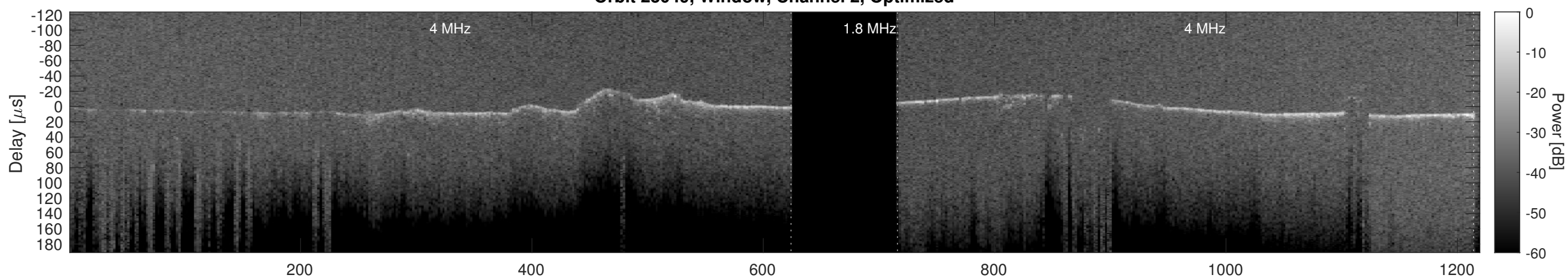
Orbit 23049, Cluttergram
