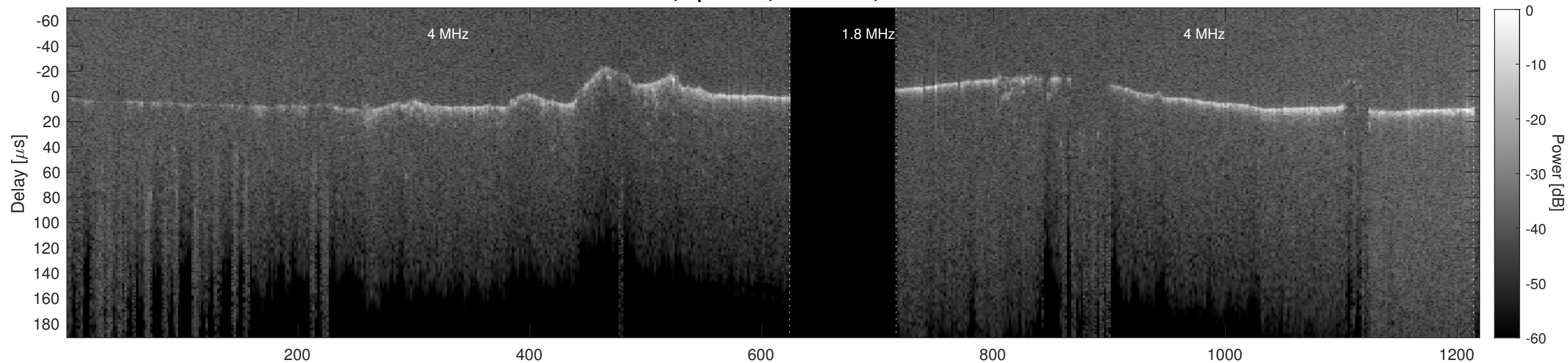
Orbit 23049, Cluttergram
