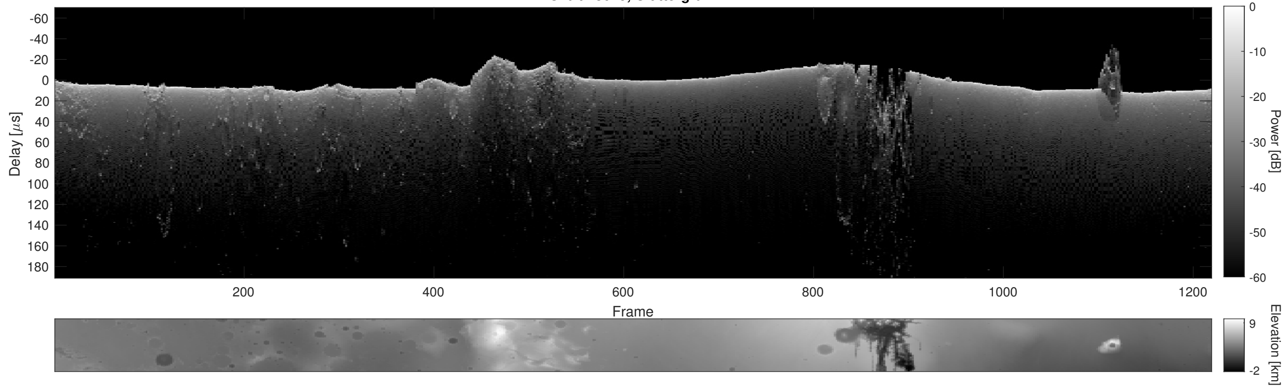
Orbit 23049, Cluttergram
