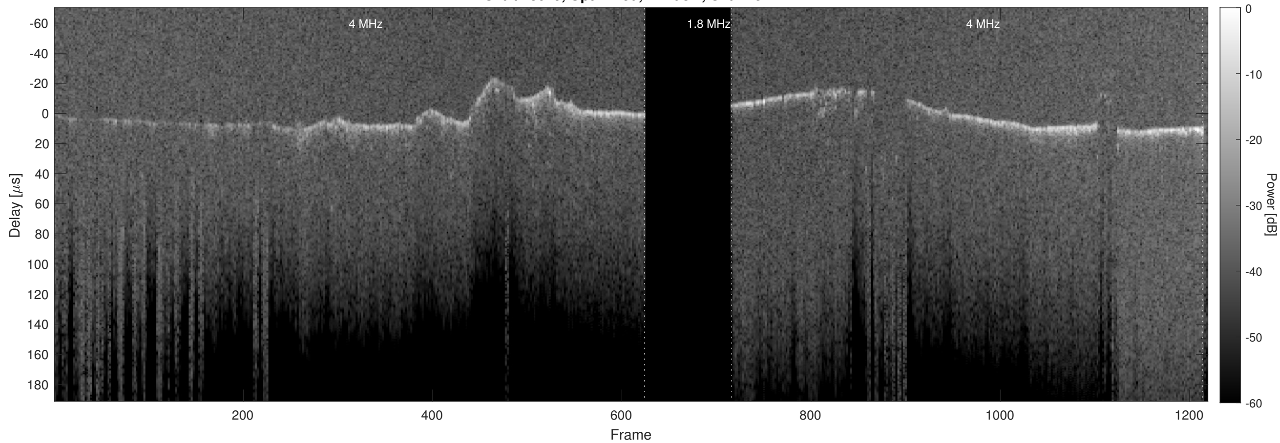
Orbit 23049, Optimized, Window, Channel 2
