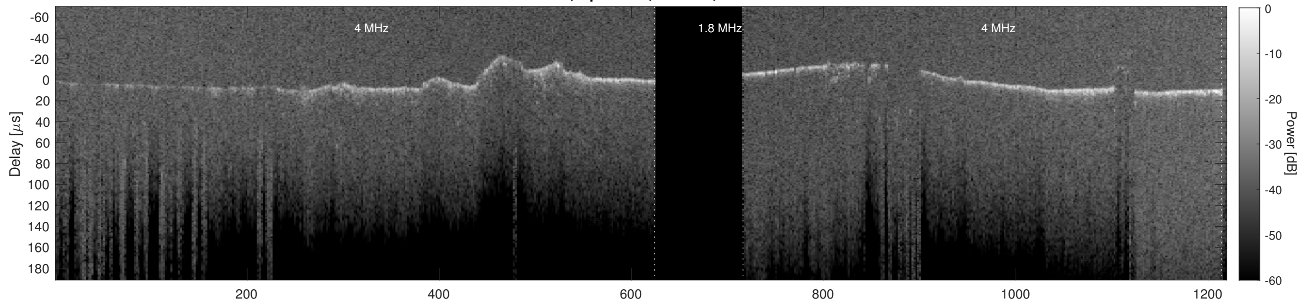
Orbit 23049, Cluttergram
