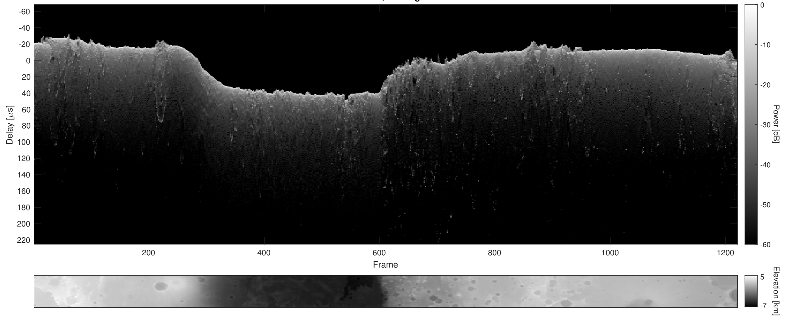
Orbit 23051, Cluttergram
