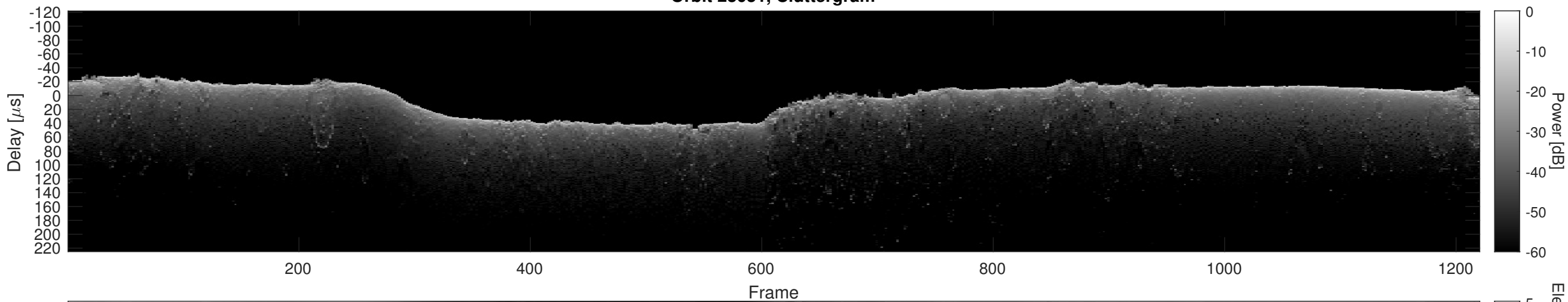
Orbit 23051, Cluttergram
