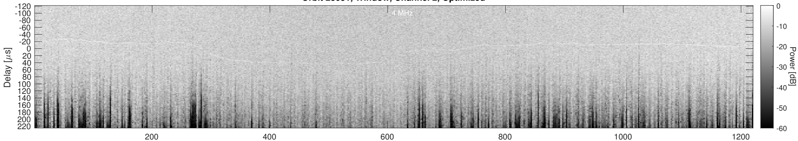
Orbit 23051, Cluttergram
