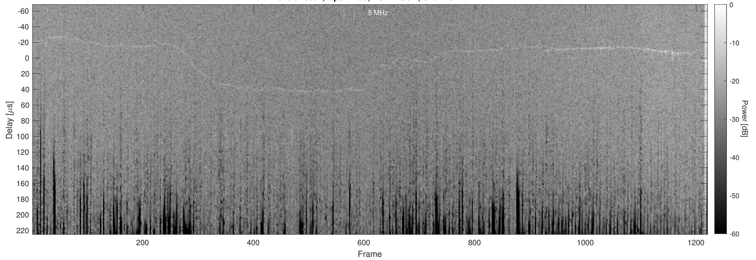
Orbit 23051, Optimized, No Window, Channel 2
