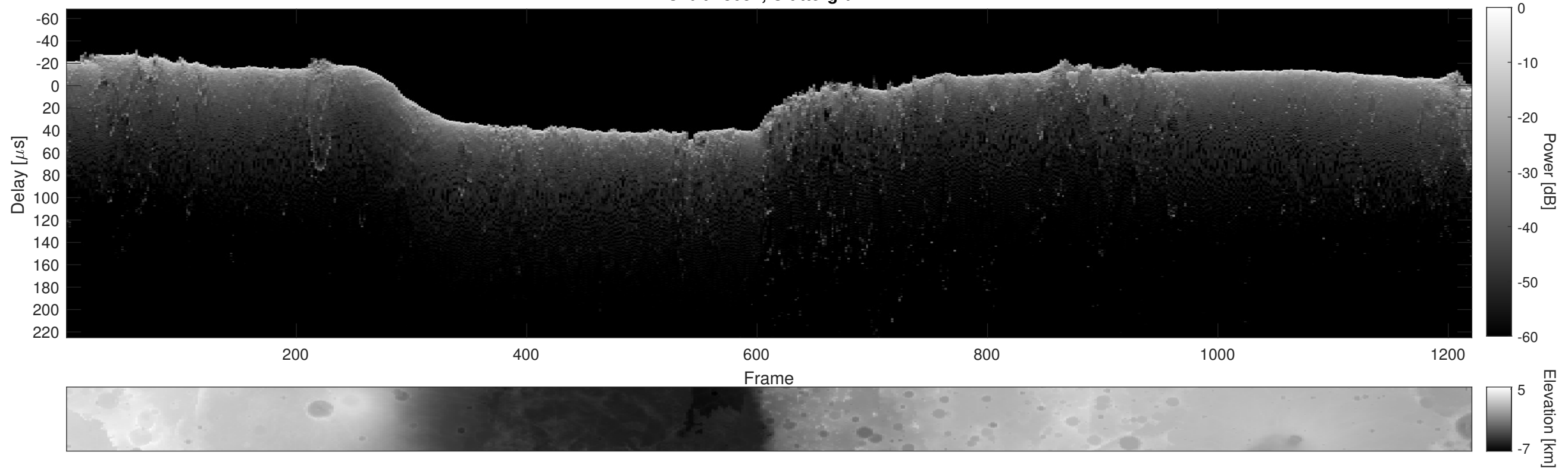
Orbit 23051, Cluttergram
