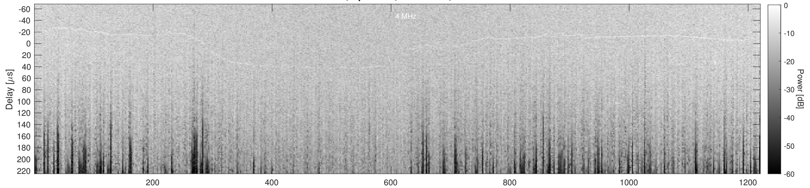
Orbit 23051, Cluttergram
