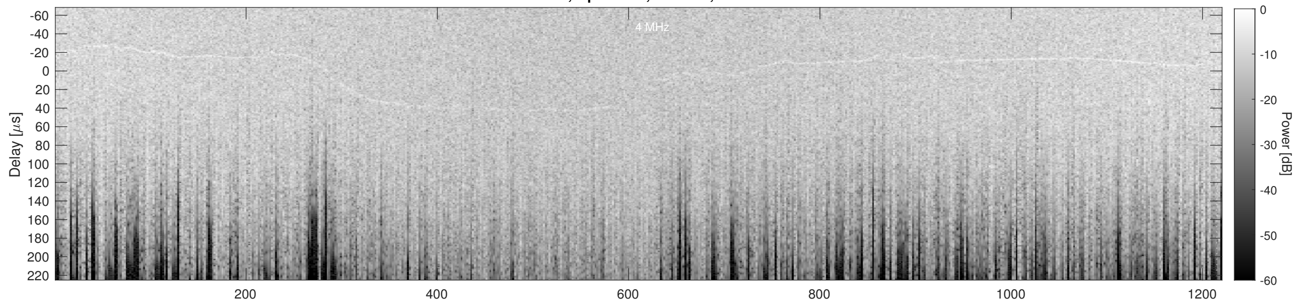
Orbit 23051, Cluttergram
