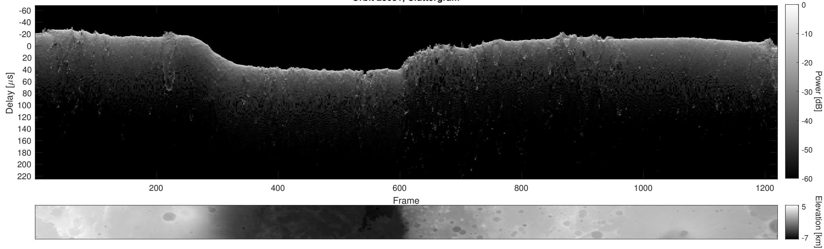
Orbit 23051, Cluttergram
