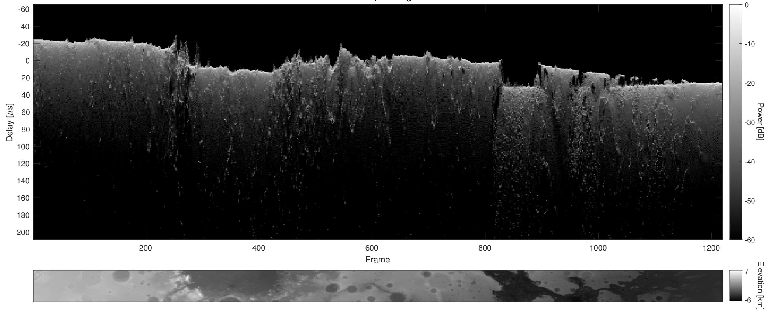
Orbit 23052, Cluttergram
