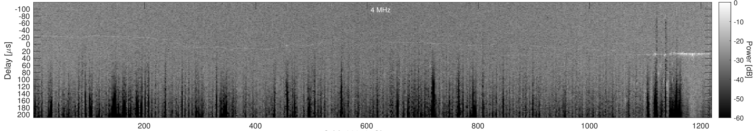
Orbit 23052, Cluttergram
