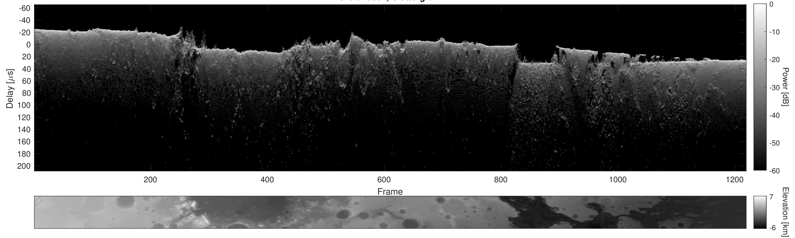
Orbit 23052, Cluttergram
