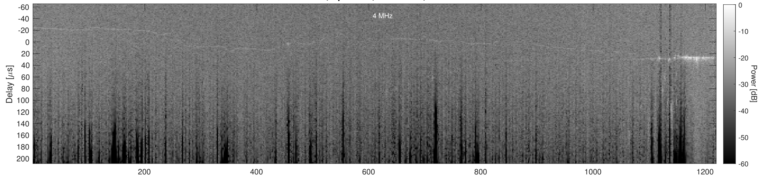
Orbit 23052, Cluttergram
