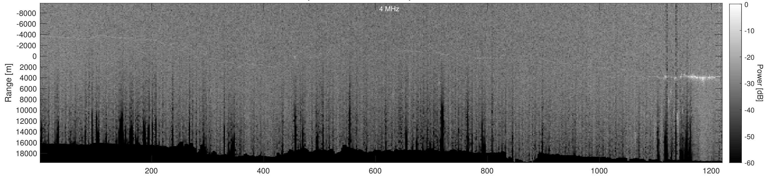
Orbit 23052, Depth-Corrected Cluttergram
