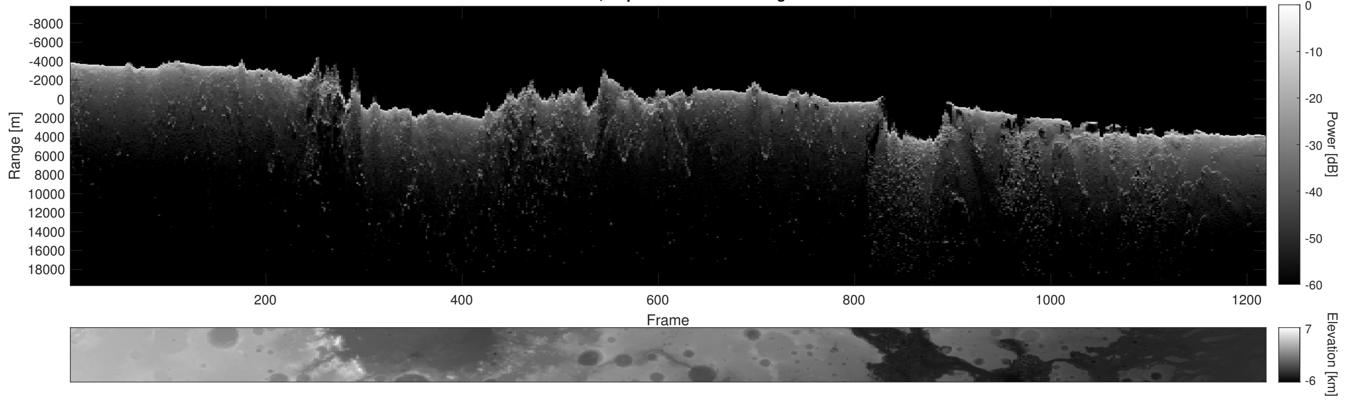
Orbit 23052, Depth-Corrected Cluttergram
