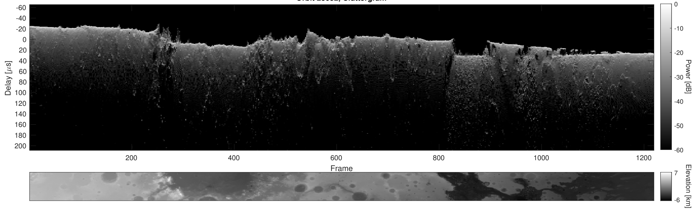
Orbit 23052, Cluttergram
