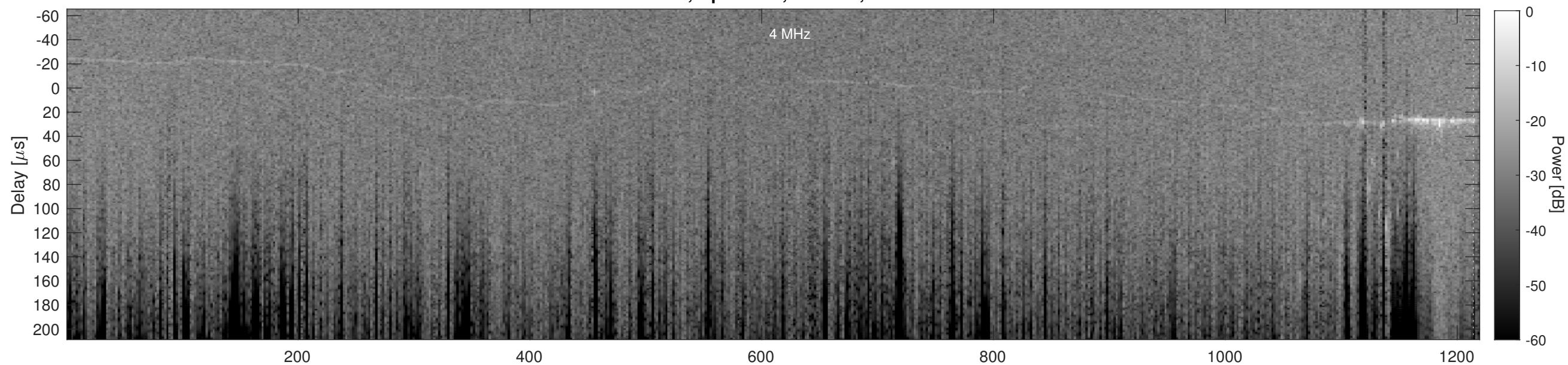
Orbit 23052, Cluttergram
