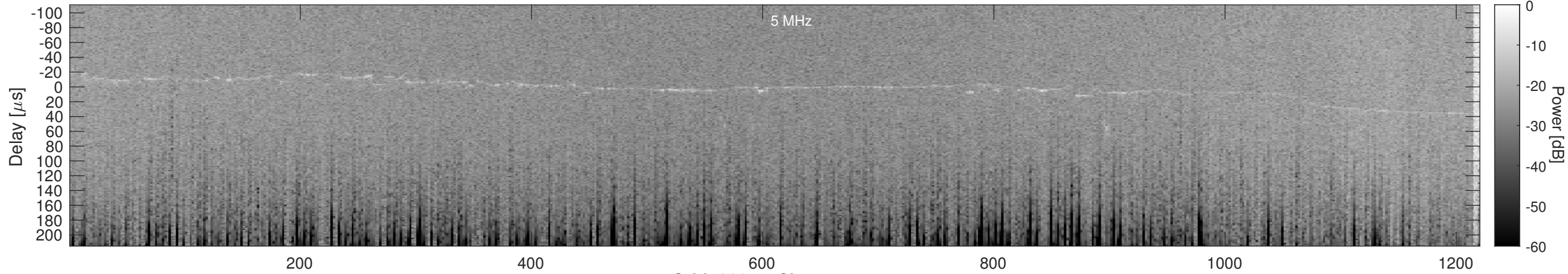
Orbit 23054, Cluttergram
