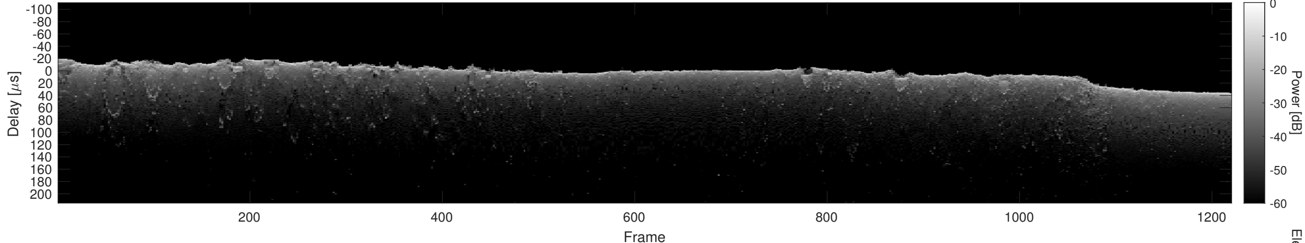
Orbit 23054, Cluttergram
