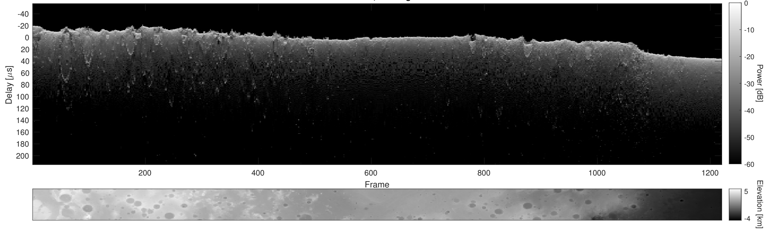
Orbit 23054, Cluttergram
