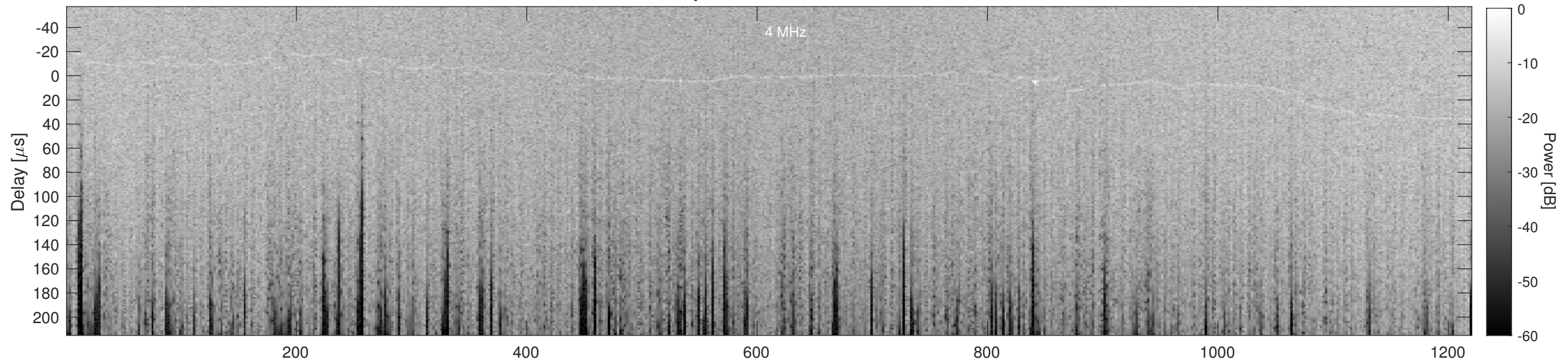
Orbit 23054, Cluttergram
