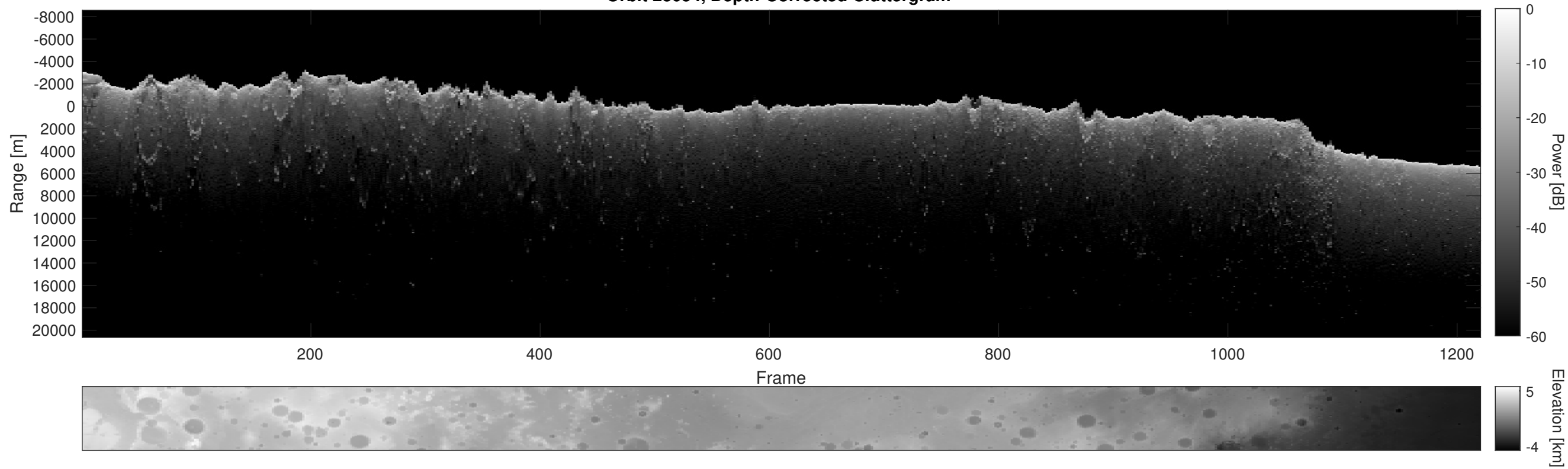
Orbit 23054, Depth-Corrected Cluttergram
