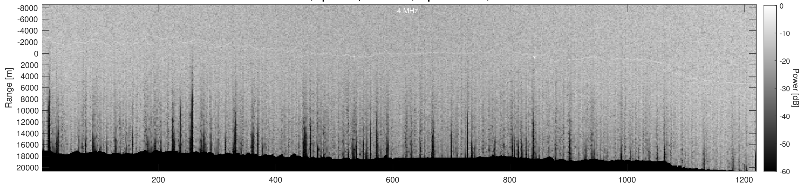
Orbit 23054, Depth-Corrected Cluttergram
