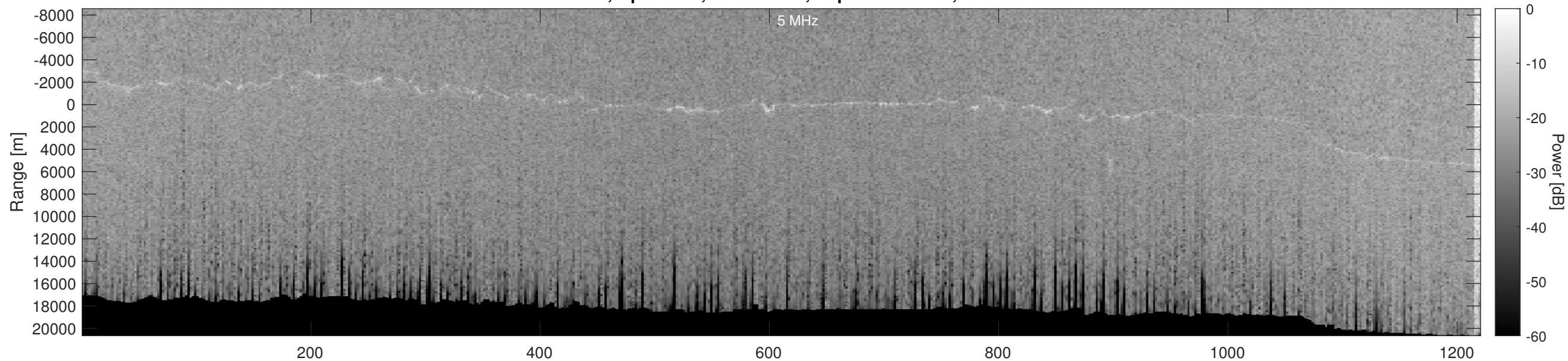
Orbit 23054, Optimized, No Window, Depth-Corrected, Channel 2
