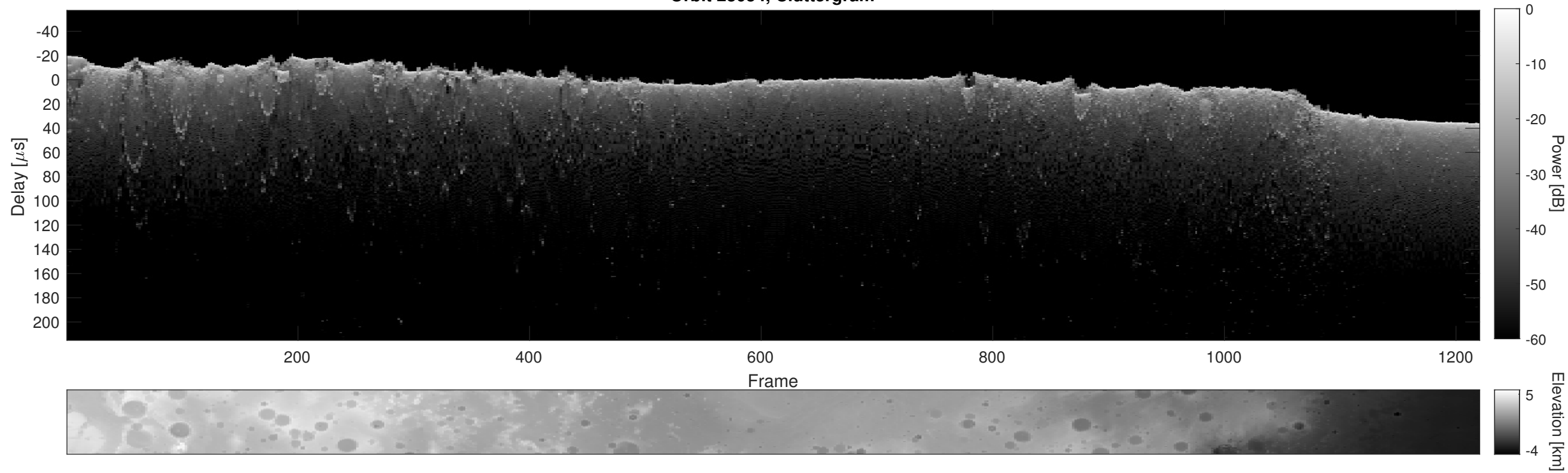
Orbit 23054, Cluttergram
