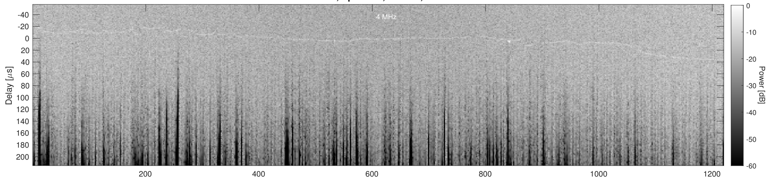
Orbit 23054, Cluttergram
