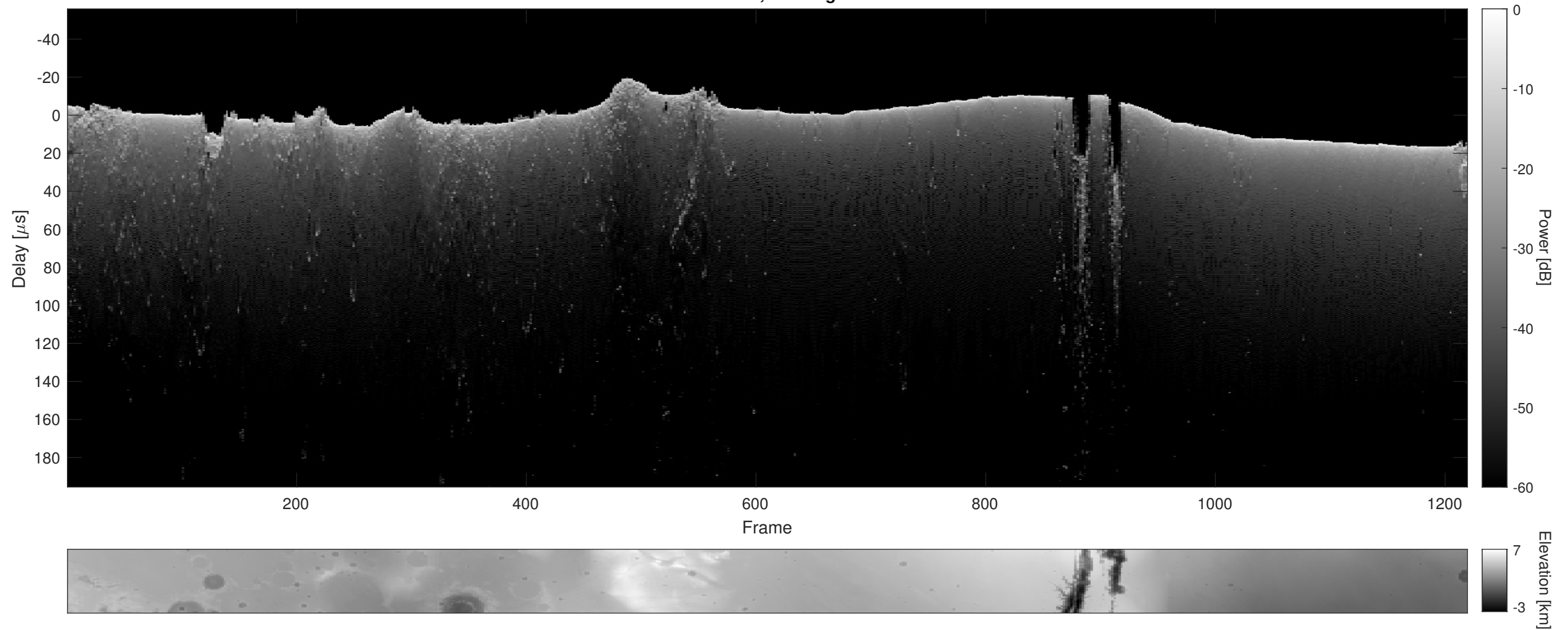
Orbit 23056, Cluttergram
