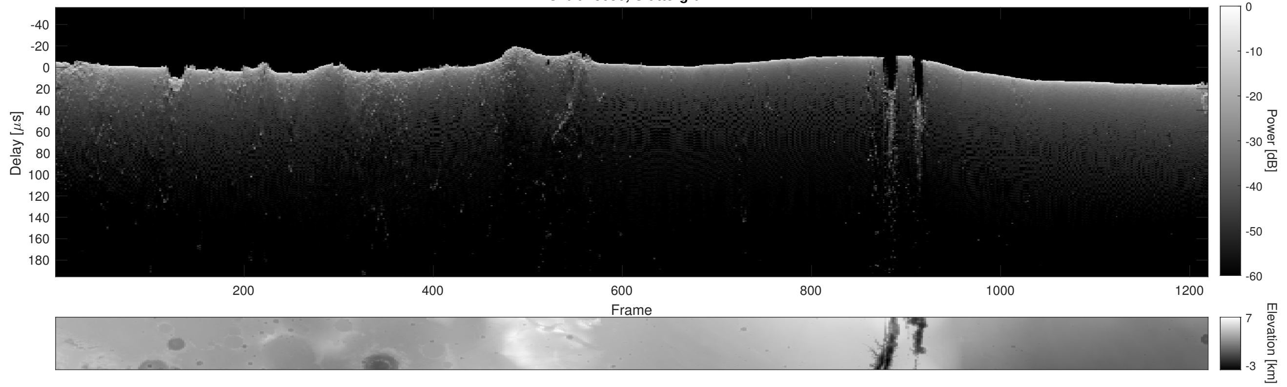
Orbit 23056, Cluttergram
