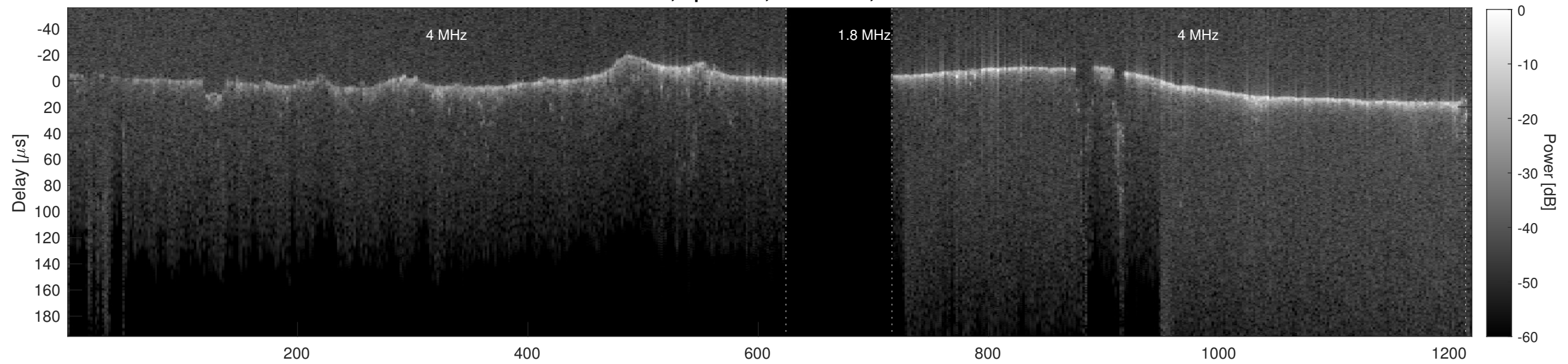
Orbit 23056, Cluttergram
