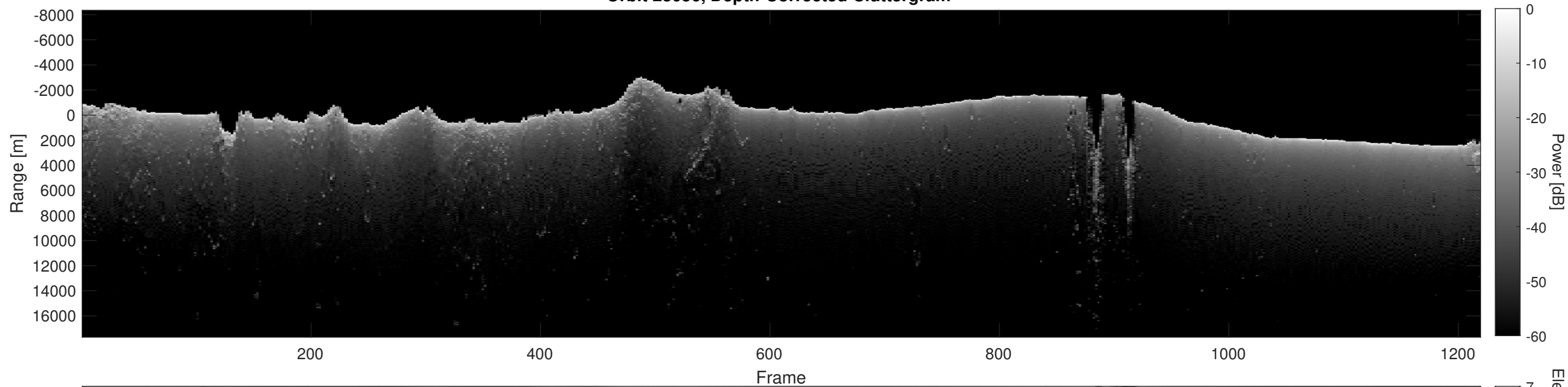
Orbit 23056, Depth-Corrected Cluttergram
