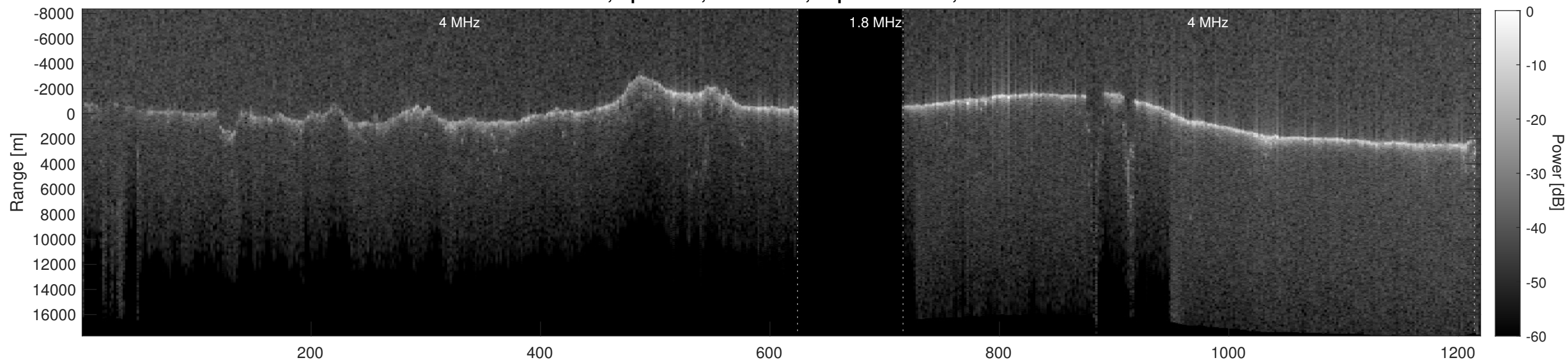
Orbit 23056, Depth-Corrected Cluttergram
