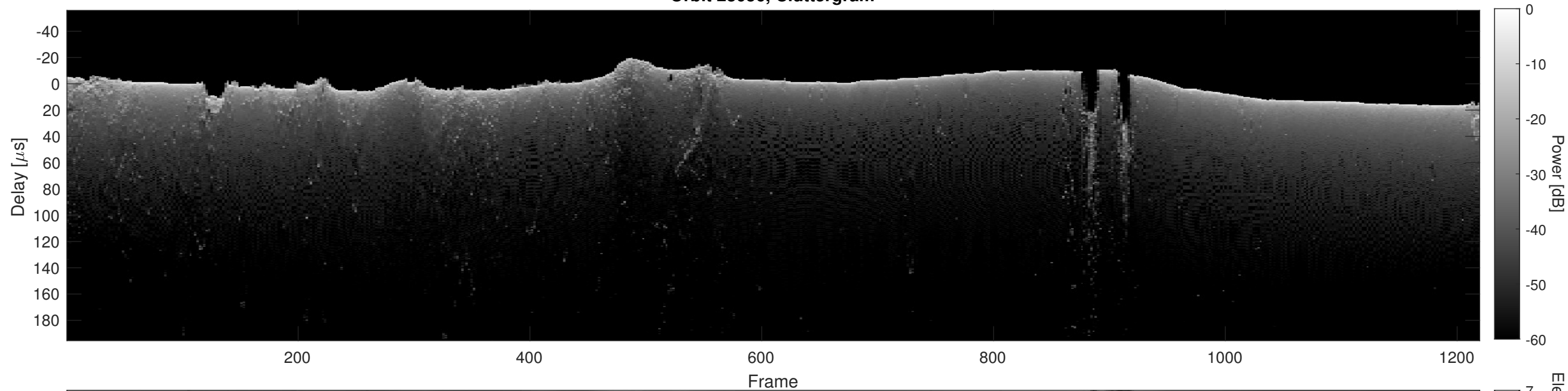
Orbit 23056, Cluttergram
