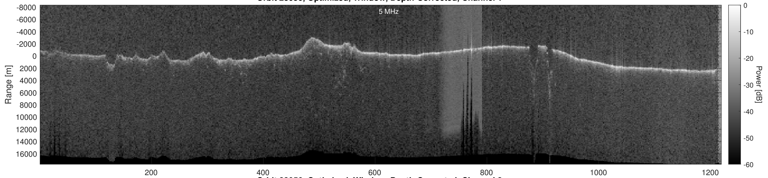
Orbit 23056, Optimized, Window, Depth-Corrected, Channel 2
