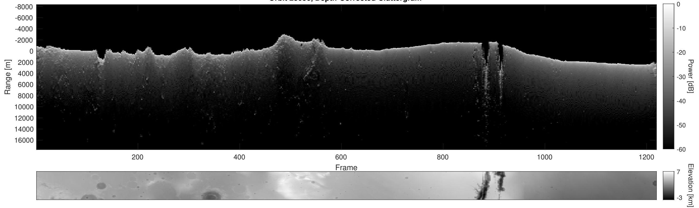
Orbit 23056, Depth-Corrected Cluttergram
