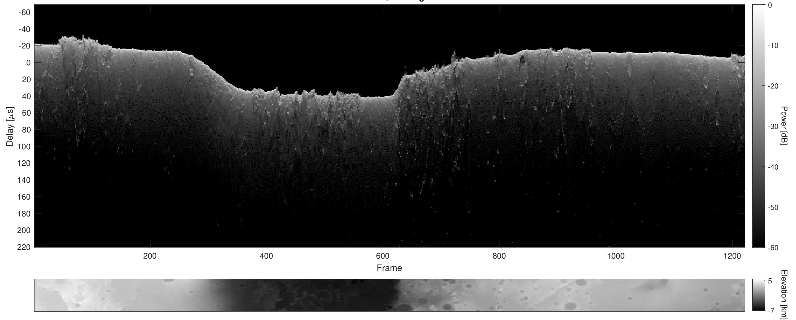
Orbit 23058, Cluttergram
