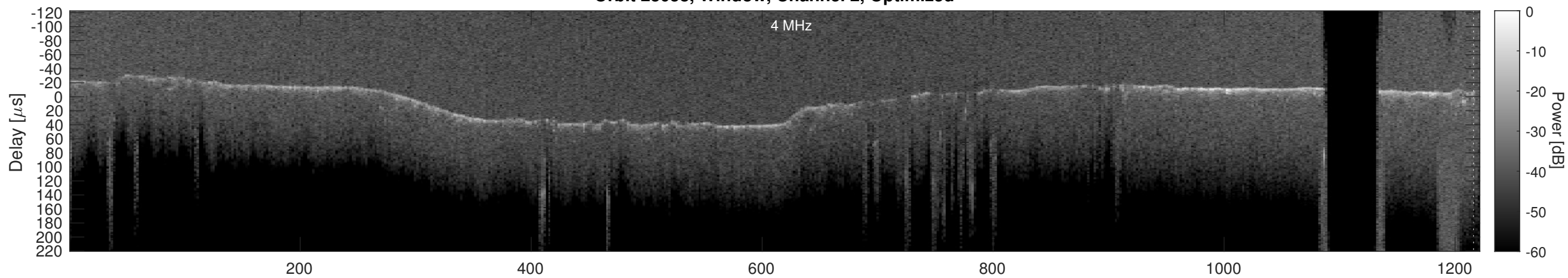
Orbit 23058, Cluttergram
