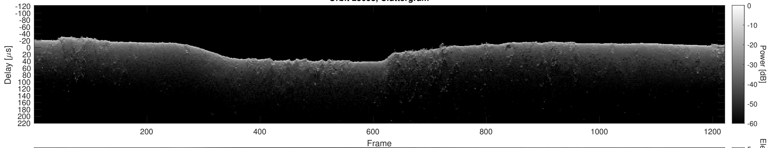
Orbit 23058, Cluttergram
