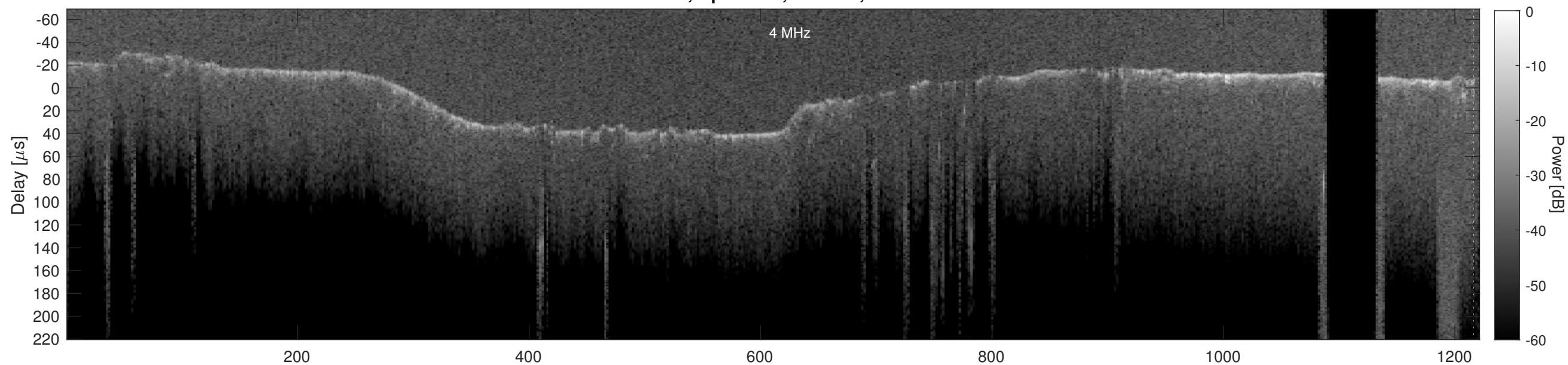
Orbit 23058, Cluttergram
