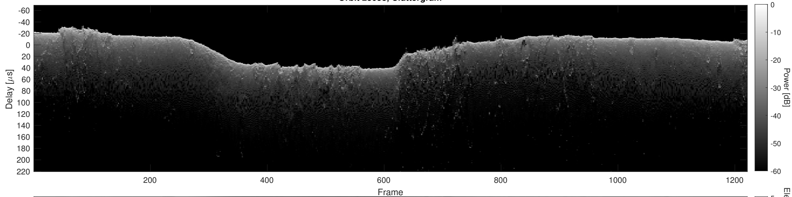
Orbit 23058, Cluttergram
