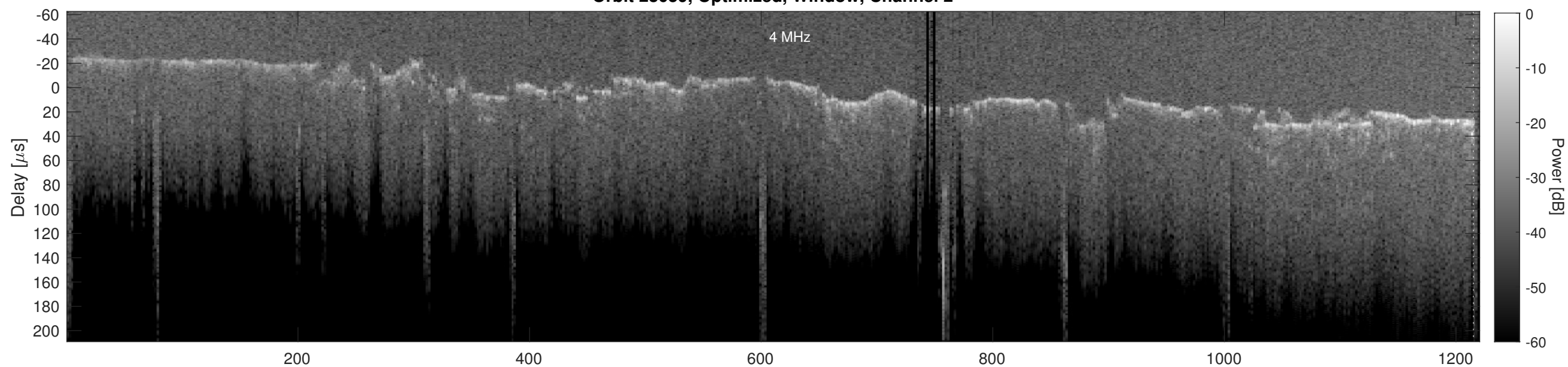
Orbit 23059, Cluttergram
