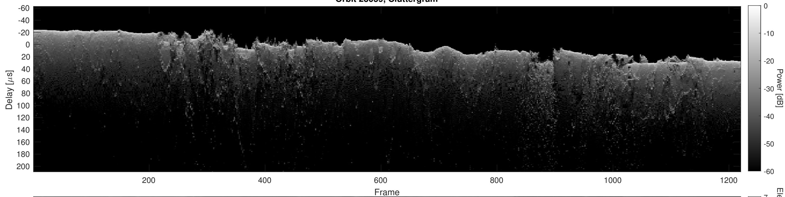
Orbit 23059, Cluttergram
