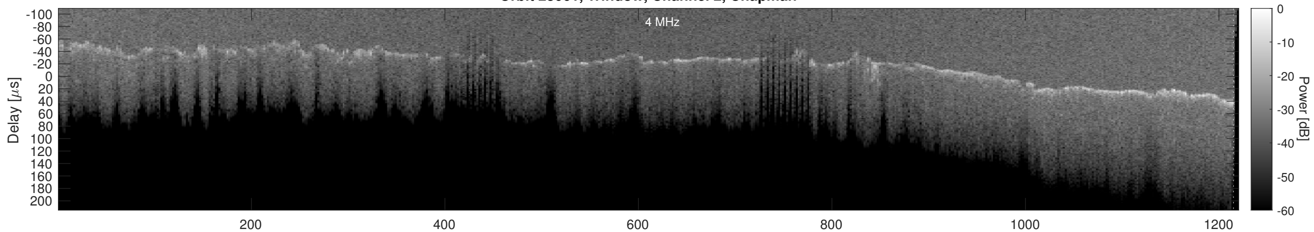
Orbit 23061, Window, Channel 2, Optimized
