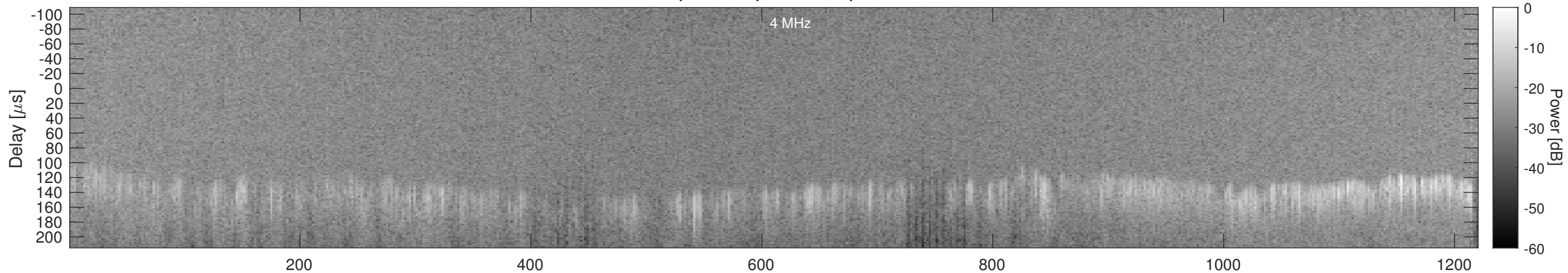
Orbit 23061, Window, Channel 2, Chapman
