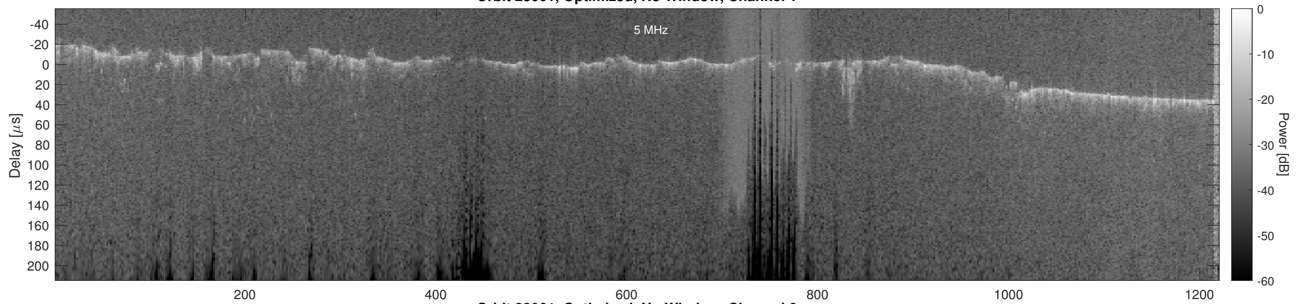
Orbit 23061, Optimized, No Window, Channel 2
