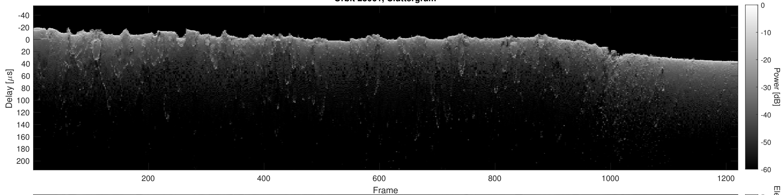
Orbit 23061, Cluttergram
