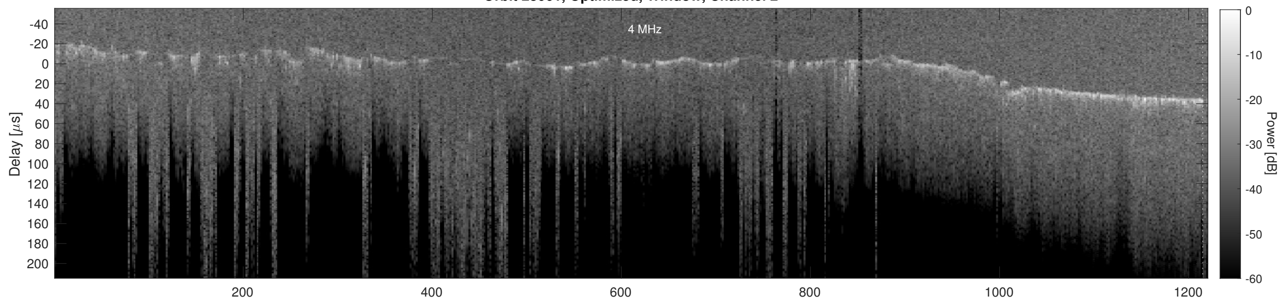
Orbit 23061, Cluttergram
