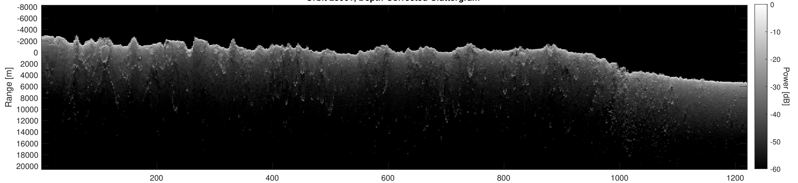
Orbit 23061, Depth-Corrected Cluttergram
